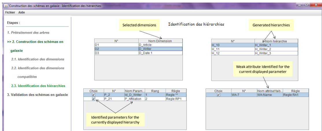
Figure 9: Galaxy-Gen interface for selecting hierarchies.
