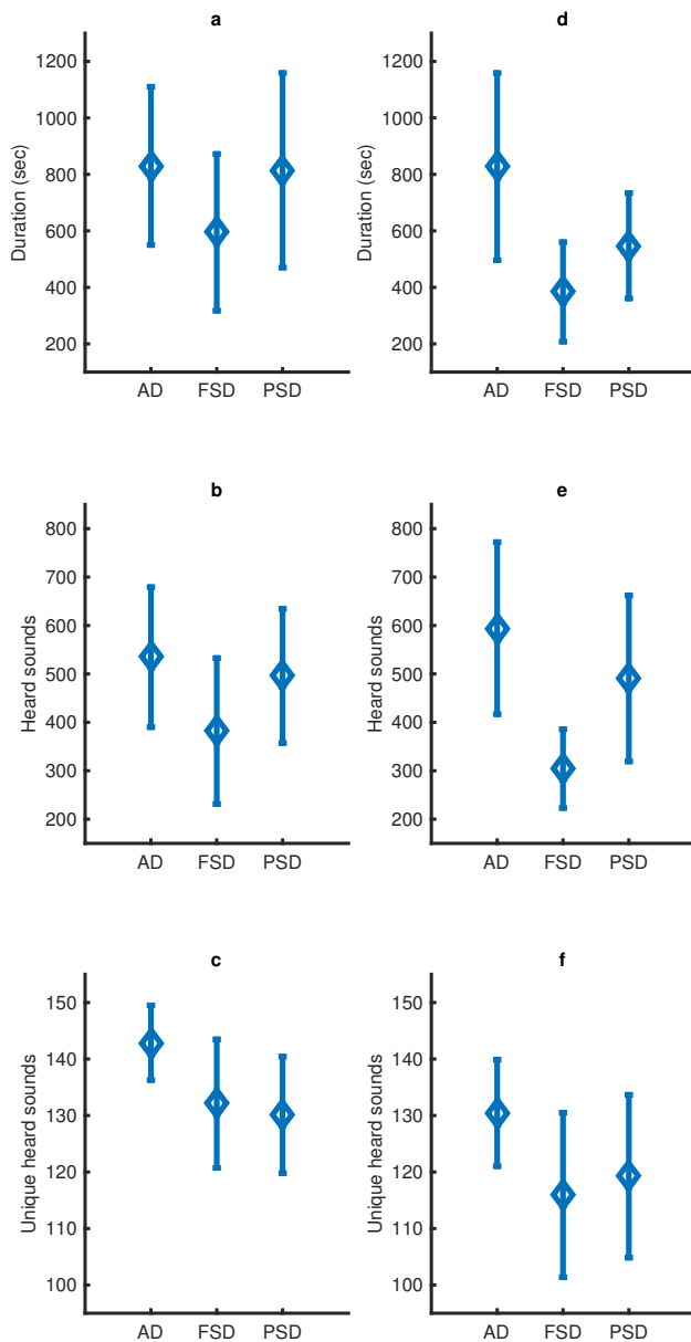
Fig. 5. Average and standard deviation for (a,d) the total search durations, (b,e) the number of heard sounds and (c,f) the number of unique heard sounds; considering respectively the urban dataset (a,b,c) and the music dataset (d,e,f).
