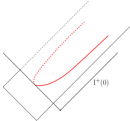
FIGURE 6. The future of a parabola is a domain of dependence invariant for the parabolic group. Its support function at infinity is lower-semicontinuous and is affine on the complement of a point of \partial\mathbb{D} .
