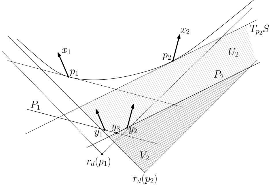
FIGURE 12. Analogously, the definitions of U_2 and V_2 . The case pictured is for y_1 \notin V_2 and y_2 \notin V_1 , hence there is a point y_3 in P_1 \cap P_2 , which lies in I^+(r_d(p_1)) \cap I^+(r_d(p_2)) .
