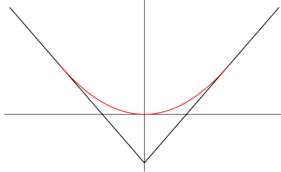
FIGURE 7. A Cauchy surface in the cone over a point, of unbounded negative curvature, which is not a spacelike entire graph. The surface (red) is obtained by revolution around the vertical axis.
