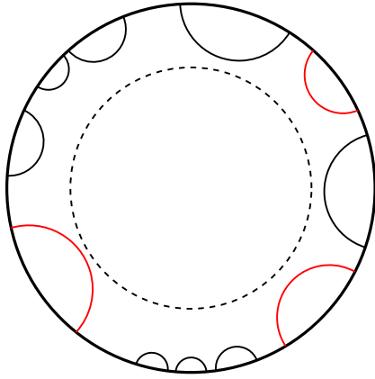
FIGURE 3. The geodesics \{g'_1, \dots, g'_{p'}\} \setminus \{g_1, \dots, g_p\} in
