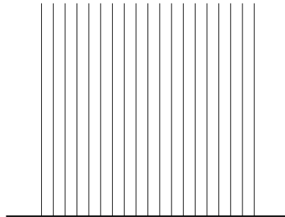
FIGURE 15. In the upper half space model, with fixed point at infinity, the measure is the Lebesgue measure.
