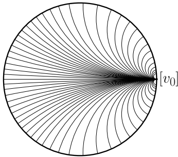
FIGURE 14. The dual lamination to the boundary of the domain of dependence, which is the future of a parabola.
