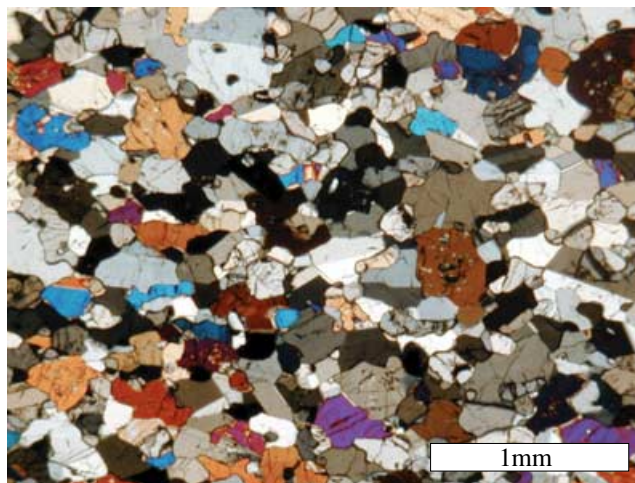
Figure 1. Optical microphotograph of the original gabbronorite sample. The rock displays a mosaic texture with polygonal plagioclase, planar to curvilinear grain boundaries, 120° triple junctions and equigranular grains, which are the expression of a microstructural equilibrium.
