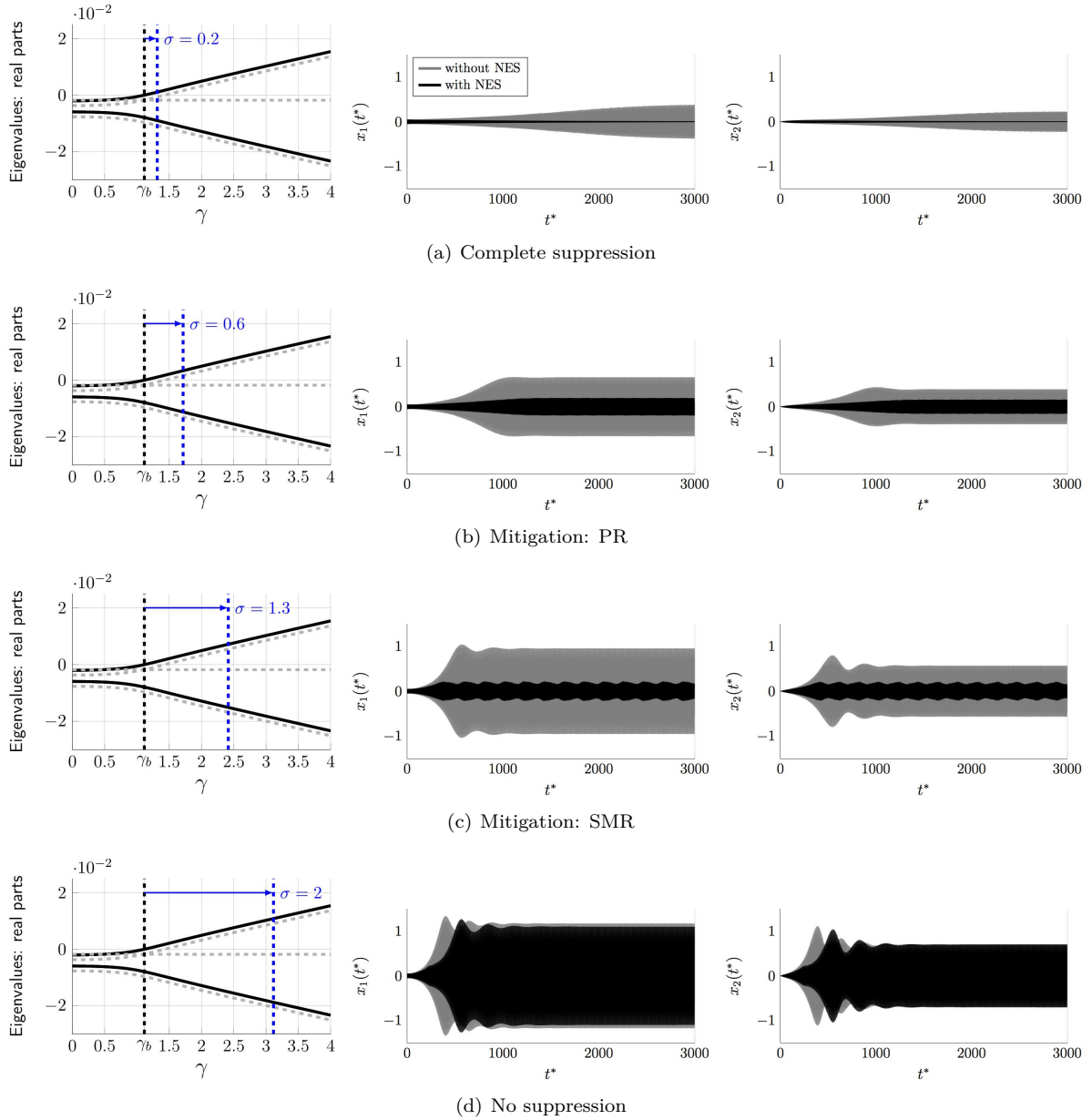
Figure 5: Comparison between time series x_1(t^*) and x_2(t^*) resulting from the numerical integration of the RHM+NES (Eqs. (6)) (solid black line) and x_1(t^*) and x_2(t^*) resulting of the numerical integration of the RPS (Eqs. (7)) (solid gray line). Set of parameters (10) is used with (a) \sigma = 0.2 , (b) \sigma = 0.6 , (c) \sigma = 1.3 and (d) \sigma = 2 . On the left, the position of each simulation in the graph representing the real parts of the eigenvalues with respect to \gamma is shown.
