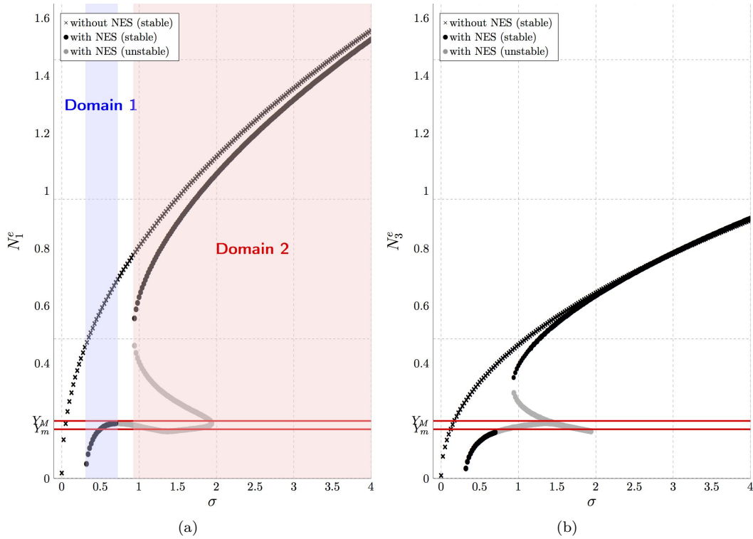
Figure 7: Comparison between the bifurcation diagrams of the slow-flow of the system without NES (RPS (7)) and with NES which is obtained from the analysis of the super-slow subsystem (50); with respect to the variable N_1 (a) and to the variable N_3 (b). Set of parameters (10) is used.
