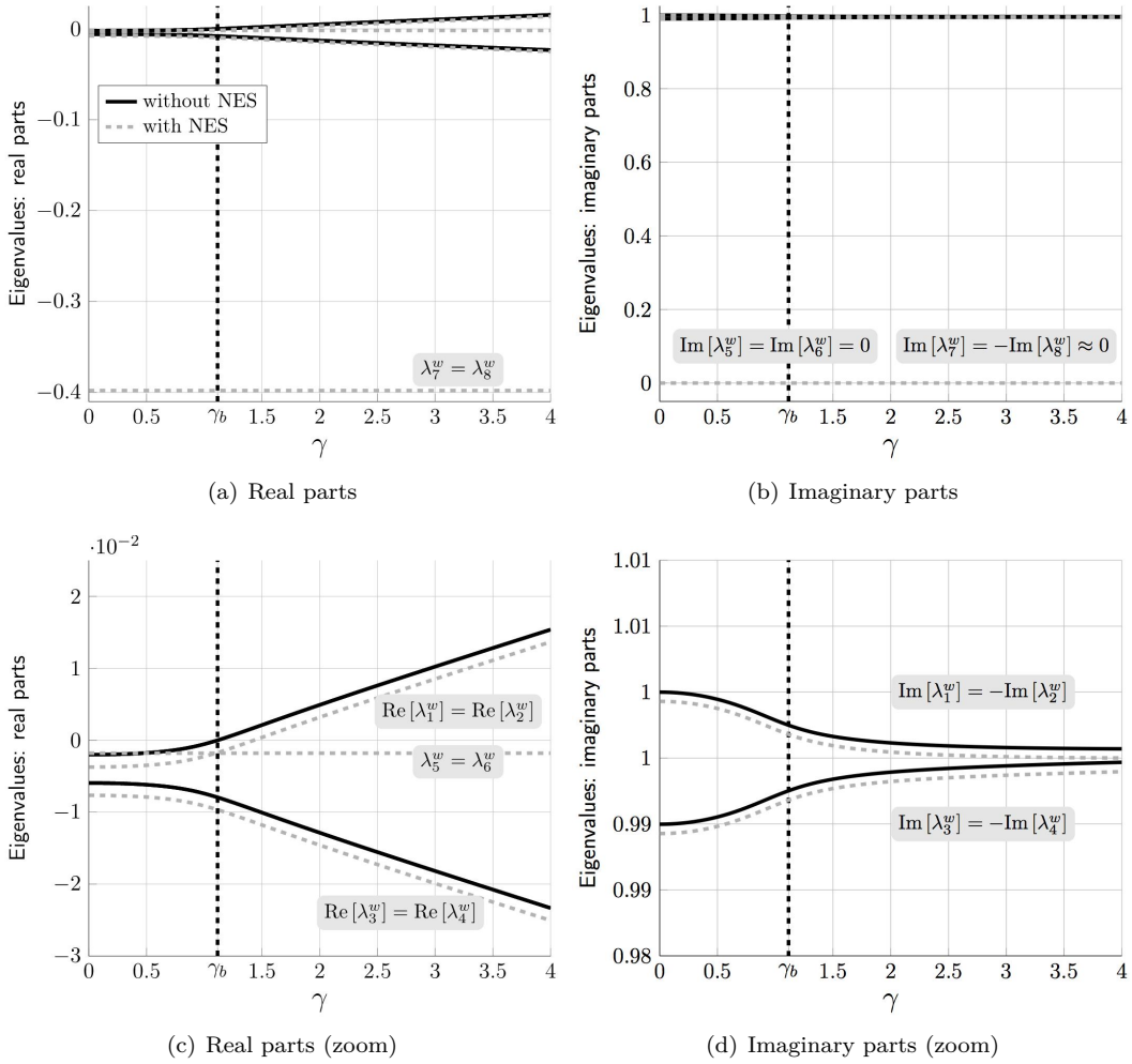
Figure 4: Evolution of real and imaginary parts of the eigenvalues of the Jacobian matrices of the vector functions \mathbf{F}_1 (solid black lines) and \mathbf{F}_2 (dashed gray lines) evaluated at the trivial equilibrium. Parameters used: a = 1 , \eta_1 = 0.4 , \eta_2 = 1.2 , \epsilon = 0.01 , \alpha_1 = 7 and \mu = 0.03 .
