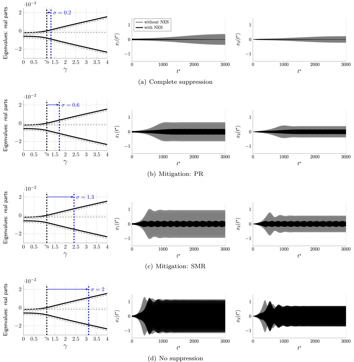
Figure 5: Comparison between time series x_1(t^*) and x_2(t^*) resulting from the numerical integration of the RHM+NES (Eqs. (6)) (solid black line) and x_1(t^*) and x_2(t^*) resulting of the numerical integration of the RPS (Eqs. (7)) (solid gray line). Set of parameters (10) is used with (a) \sigma = 0.2 , (b) \sigma = 0.6 , (c) \sigma = 1.3 and (d) \sigma = 2 . On the left, the position of each simulation in the graph representing the real parts of the eigenvalues with respect to \gamma is shown.
