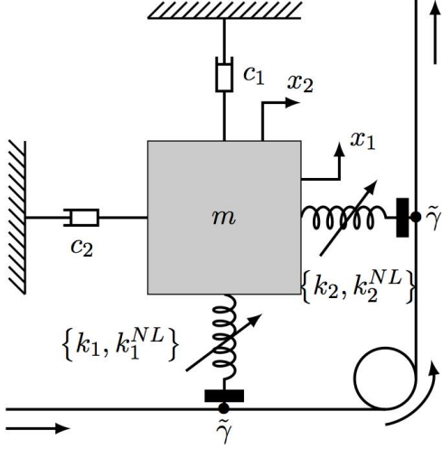
Figure 1: Mechanical system without NES.
