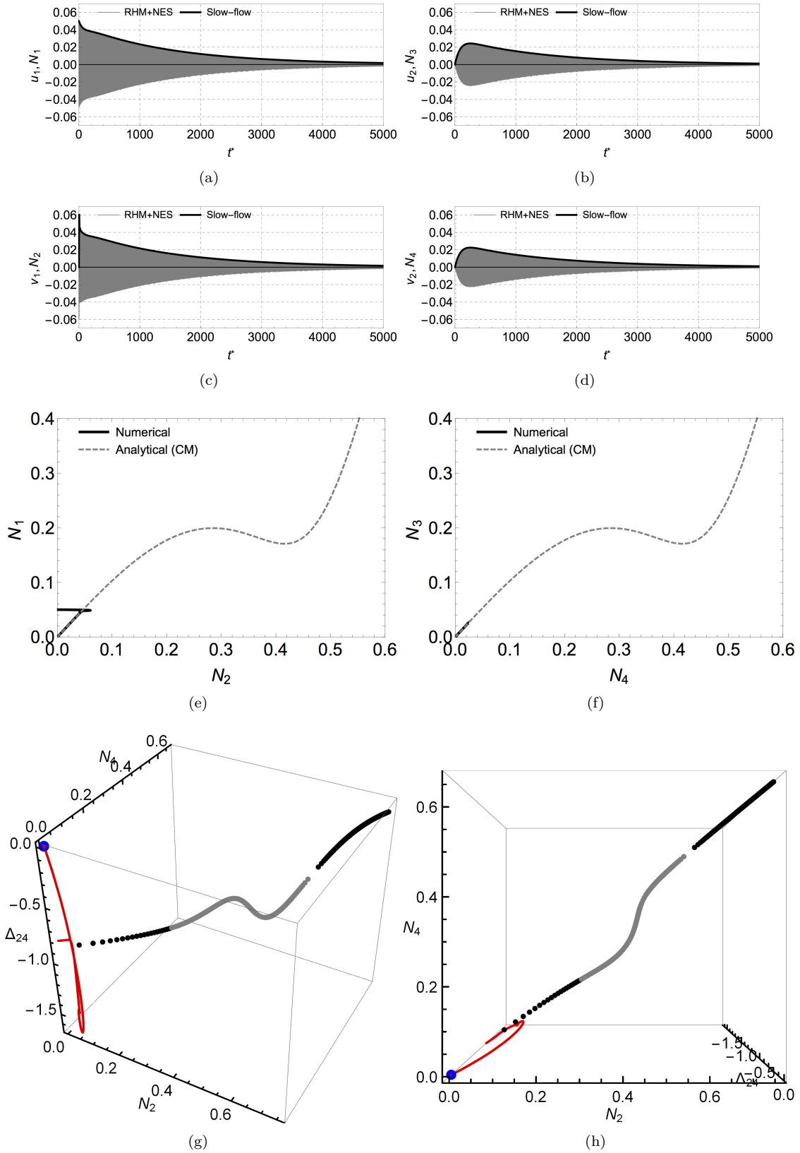
Figure 10: (a), (b), (c) and (d) compare numerical simulations of the RHM+NES written using barycentric coordinates (see Eq. (17)) (solid grey line) and numerical simulations of the slow-flow (21) (solid black line). (e) and (f) compare the Critical Manifold N_1 = \sqrt{H(N_2)} and N_3 = \sqrt{H(N_4)} (dashed grey line) (see Eq. (32)) with numerical simulations of the slow-flow (solid black line). (g) and (h) compare the bifurcation diagram obtained from Eq. (53) (black and grey points for stable and unstable branches respectively) with the trajectory of the slow-flow (solid red line) in the 3D N_2, N_4, \Delta_{25} -space. The blue point shows the initial condition and two views are used to make the reading of the 3D graph easier. Set of parameters (10) is used and \sigma = 0.2 .
