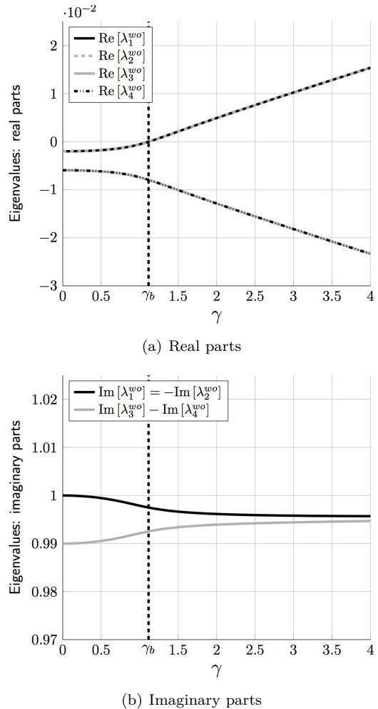
Figure 3: Evolution of real and imaginary parts of the eigenvalues of the Jacobian matrix of the vector function \mathbf{F}_1 evaluated at the trivial equilibrium. Parameters used: a = 1 , \eta_1 = 0.4 , \eta_2 = 1.2 and \epsilon = 0.01 . \gamma_b is the Hopf bifurcation point.
