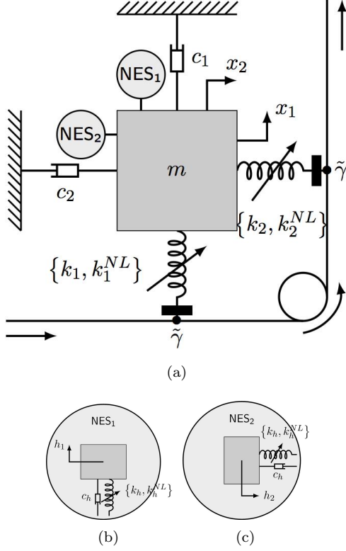
Figure 2: (a) Mechanical system with NES. (b) Zoom on the NES 1 . (c) Zoom on the NES 2 .
