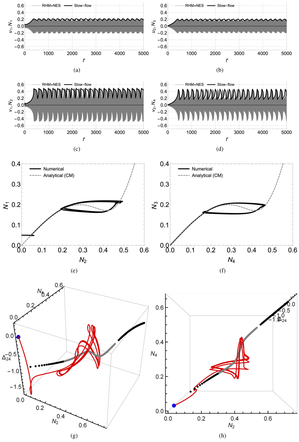
Figure 13: Same caption as for Fig. 10. Set of parameters (10) is used and \sigma = 1.3 .
