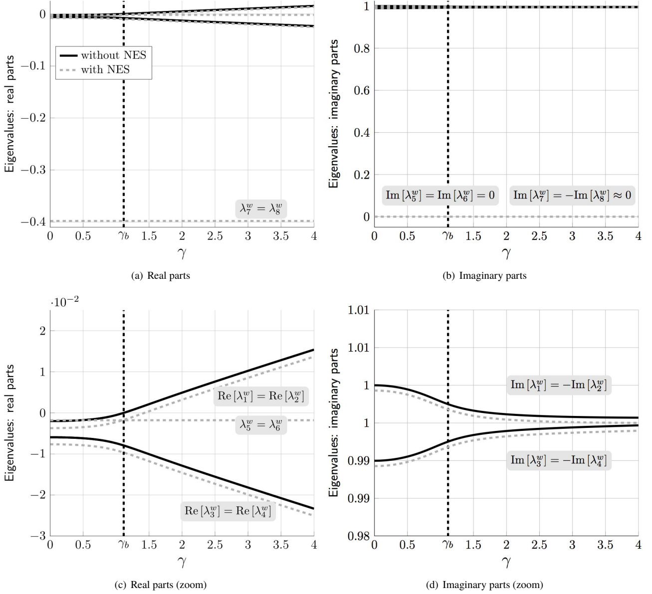
Figure 4: Evolution of real and imaginary parts of the eigenvalues of the Jacobian matrices of the vector functions \mathbf{F}_1 (solid black lines) and \mathbf{F}_2 (dashed gray lines) evaluated at the trivial equilibrium. Parameters used: a = 1 , \eta_1 = 0.4 , \eta_2 = 1.2 , \epsilon = 0.01 , \alpha_1 = 7 and \mu = 0.03 .
