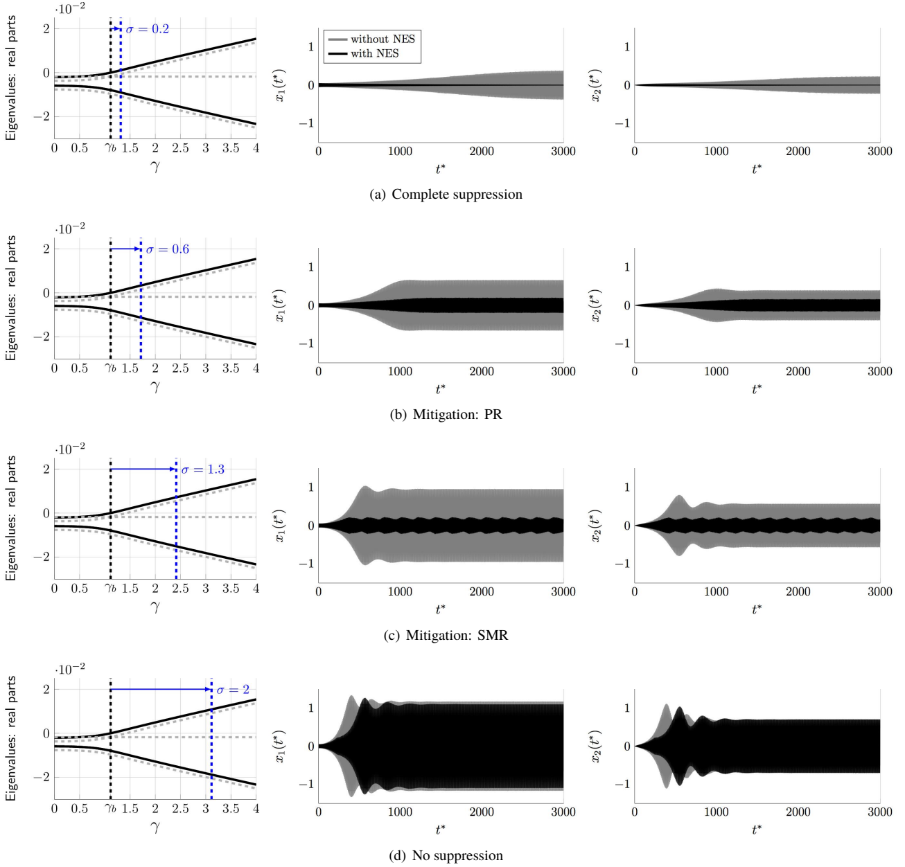
Figure 5: Comparison between time series x_1(t^*) and x_2(t^*) resulting from the numerical integration of the RHM+NES (Eqs. (6)) (solid black line) and x_1(t^*) and x_2(t^*) resulting from the numerical integration of the RPS (Eqs. (7)) (solid gray line). Set of parameters (10) is used with (a) \sigma = 0.2 , (b) \sigma = 0.6 , (c) \sigma = 1.3 and (d) \sigma = 2 . On the left, the position of each simulation in the graph representing the real parts of the eigenvalues with respect to \gamma is shown.
