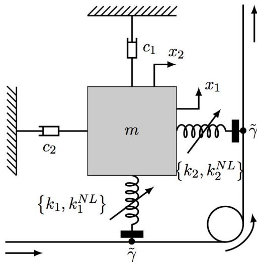
Figure 1: Mechanical system without NES.
