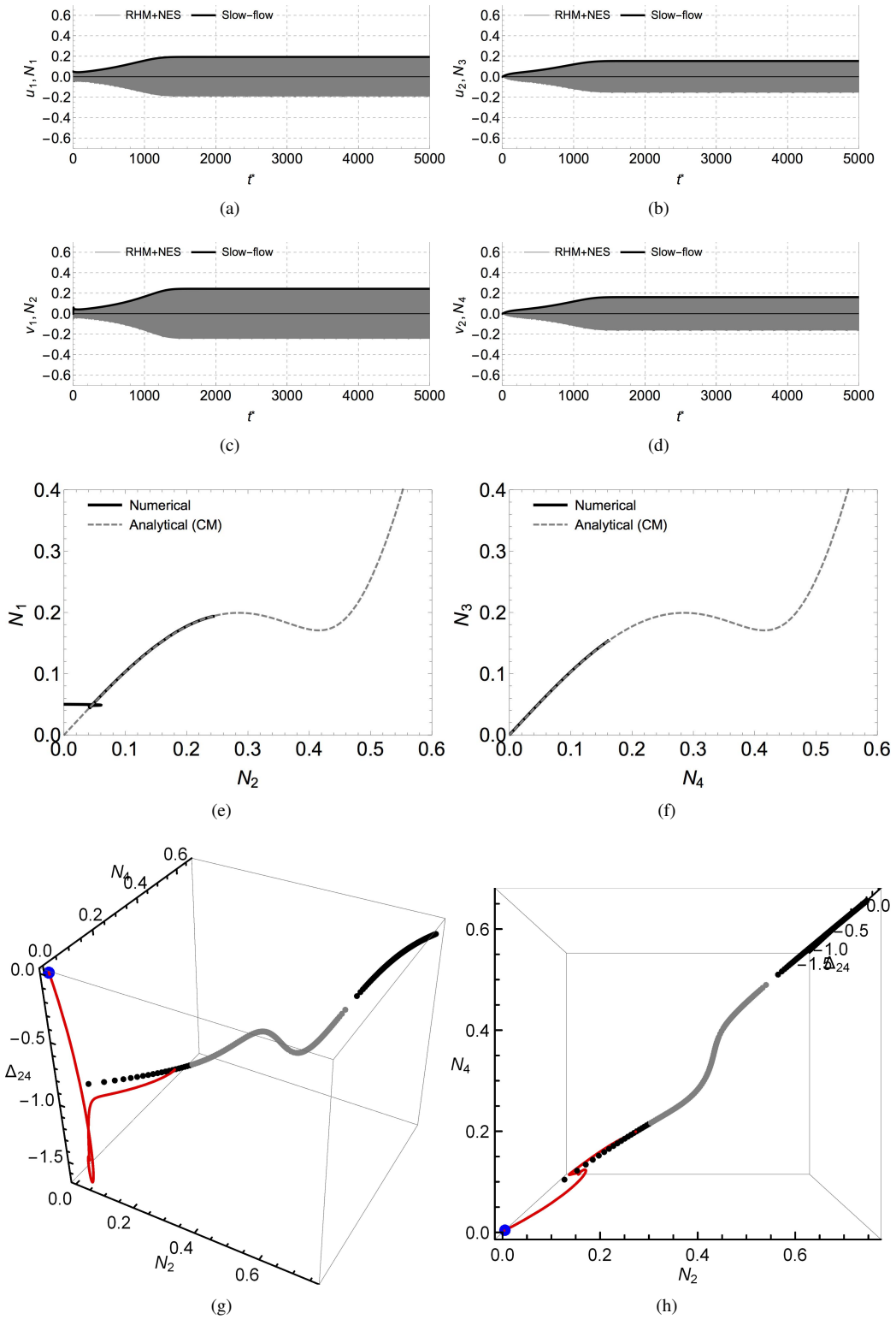
Figure 11: Same caption as for Fig. 10. Set of parameters (10) is used and \sigma = 0.6 .
