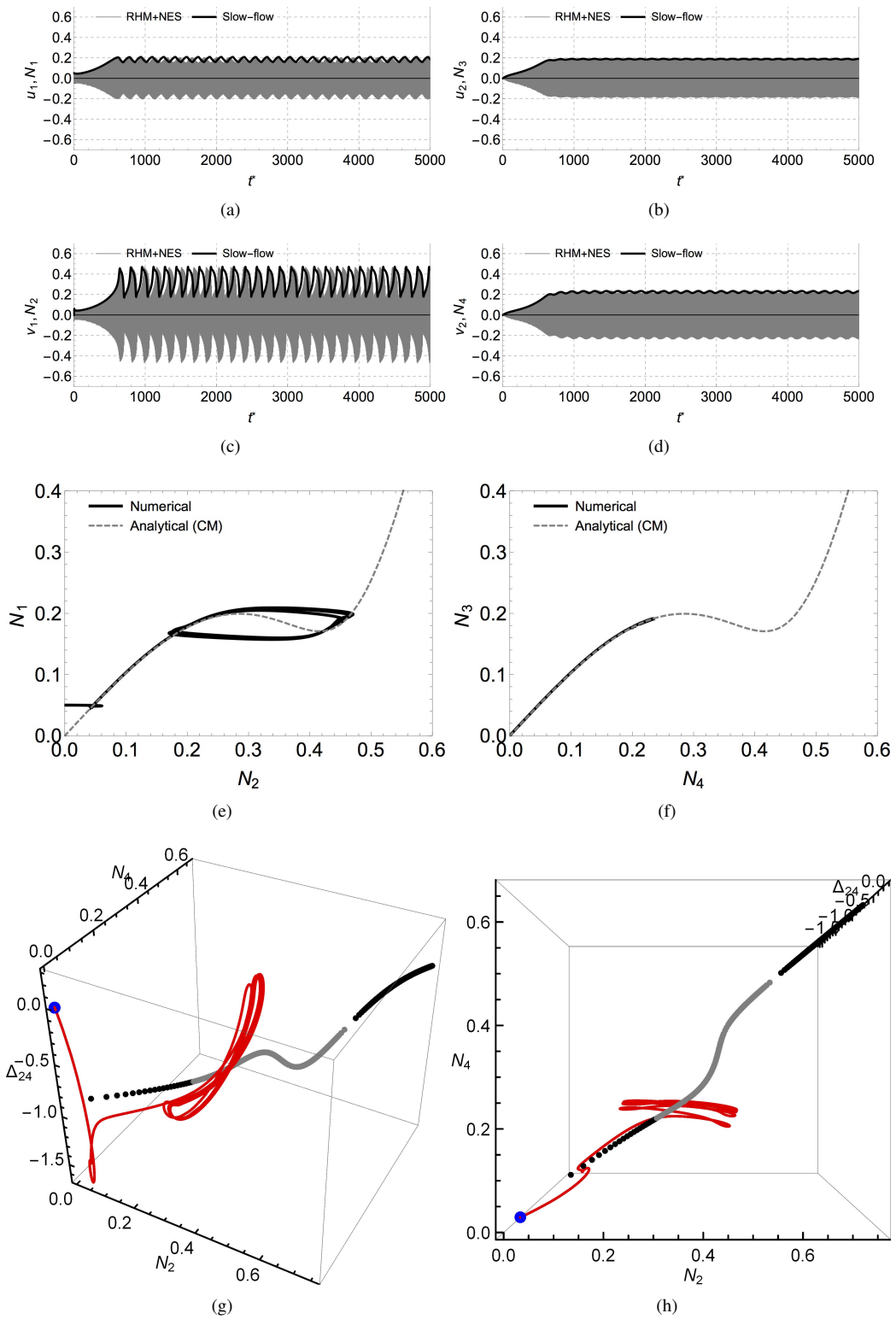
Figure 12: Same caption as for Fig. 10. Set of parameters (10) is used and \sigma = 0.9 .
