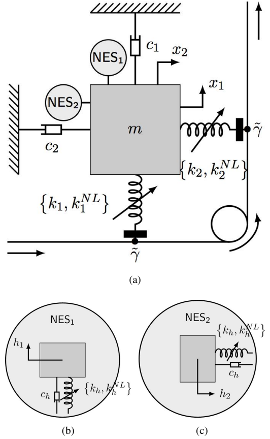
Figure 2: (a) Mechanical system with NES. (b) Zoom on the NES 1 . (c) Zoom on the NES 2 .
