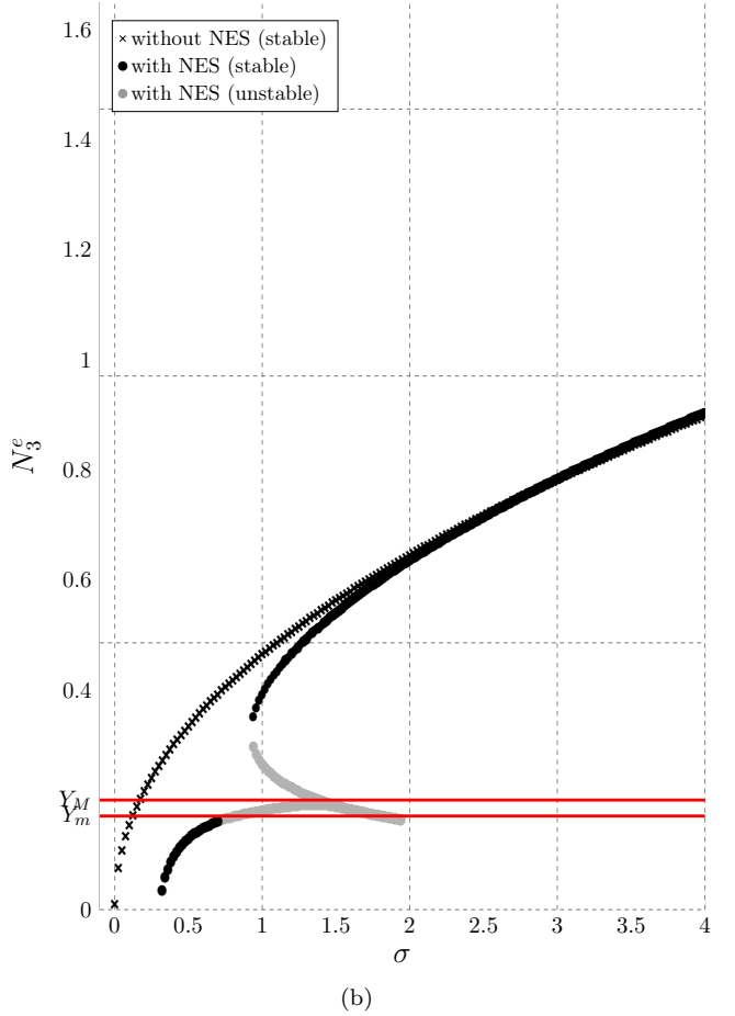
Figure 7: Comparison between the bifurcation diagrams of the slow-flow of the system without NES (RPS (7)) and with NES which is obtained from the analysis of the super-slow subsystem (50); with respect to the variable N_1 (a) and to the variable N_3 (b). Set of parameters (11) is used.
