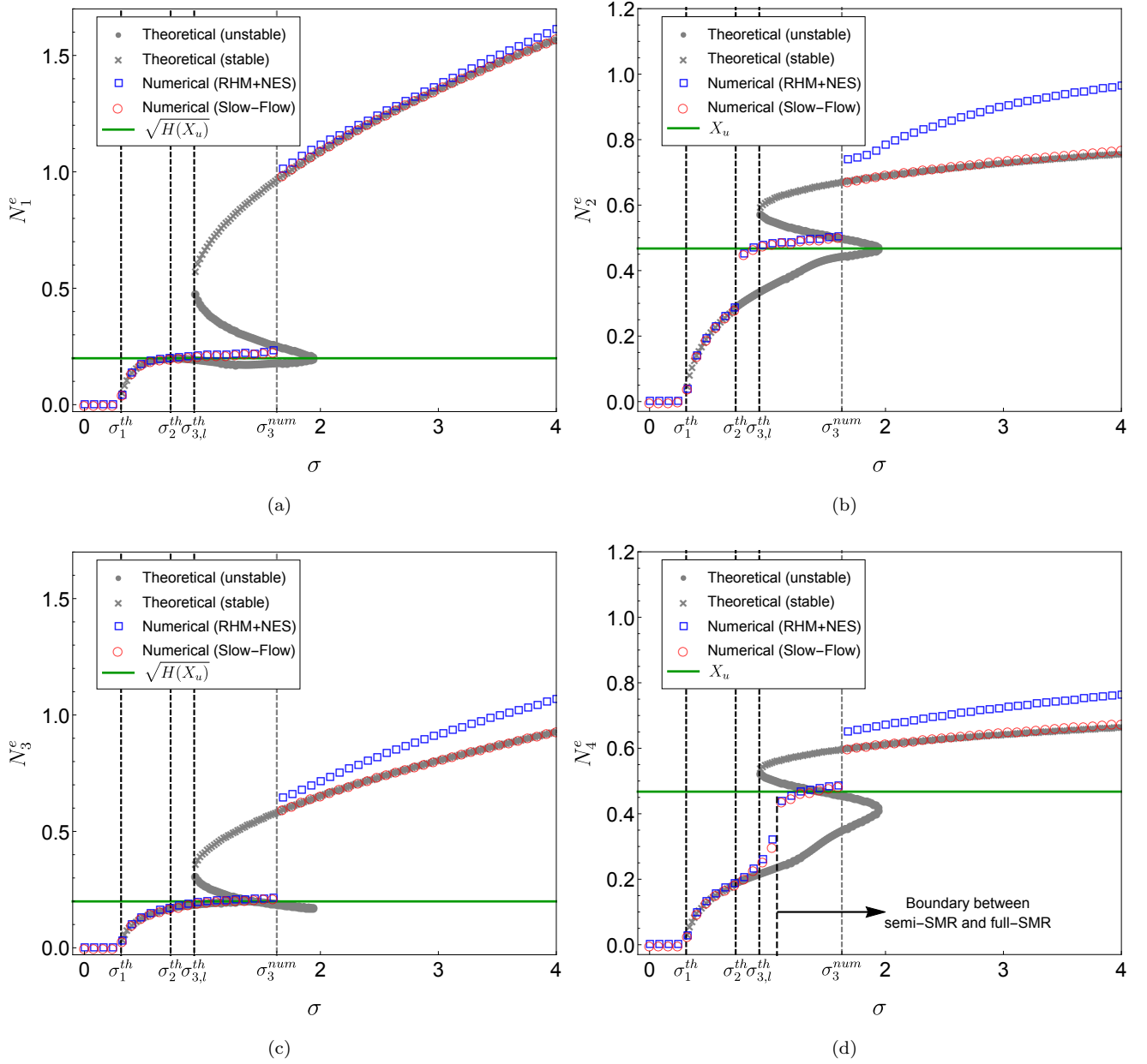
Figure 15: Comparison between steady-state amplitudes obtained from numerical simulations of the RHM+NES written using barycentric coordinates (see Eq. (17)) (blue squares) and from numerical simulations of the slow-flow (21) (red circles). Set of parameters (11) is used.
