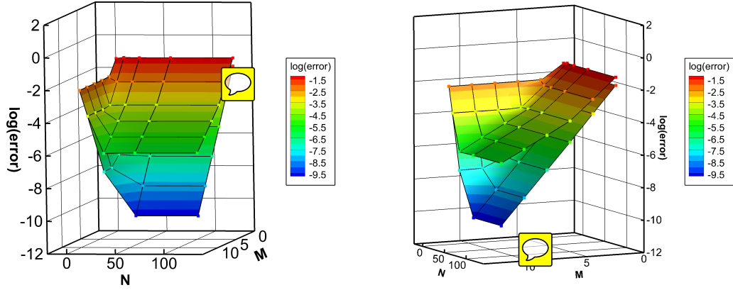
Figure 5: Error on the vertical velocity in function of N and M - kh=0.916 and ka=0.1 . Lower-surface : \frac{\beta}{h_0} = 0\% . Higher-surface : \frac{\beta}{h_0} = 25\% .
