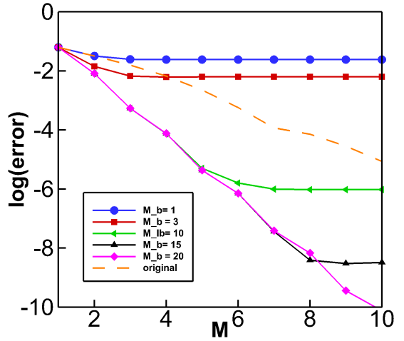
Figure 13: Error on the vertical velocity as function of M and M_b - \frac{\beta}{h_0} = 40\% - kh = 3 and ka = 0.1 .
