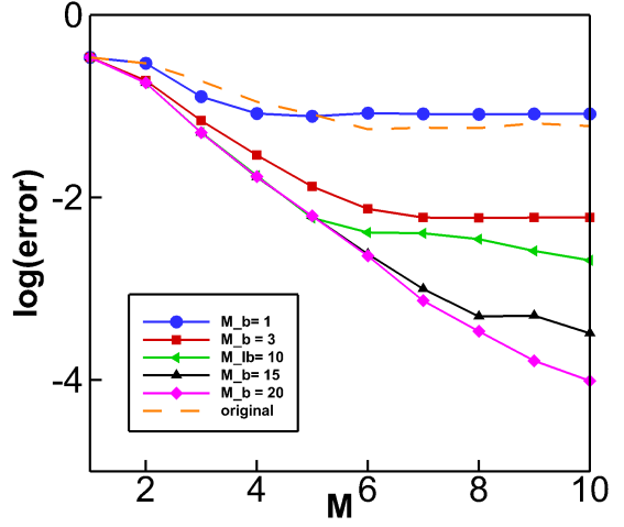
Figure 11: Error on the vertical velocity as function of M and M_b - \frac{\beta}{h_0} = 75\% - kh = 0.916 and ka = 0.15 .
