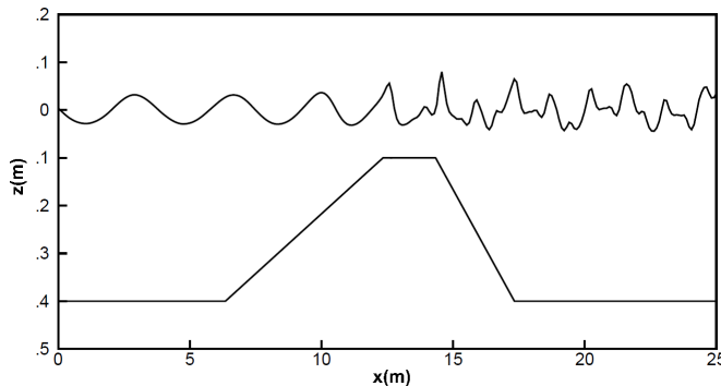
Figure 20: Snapshot of the surface elevation at a steady-state (scaled by a factor of 3).
