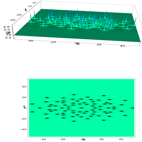
Figure 10: Solution of NLS, N=11 , \tilde{a}_5 = 10^{11} : 6 rings of 11, 11, 22, 11, 11, 11 peaks one peak in the center; on the right, sight from top.
