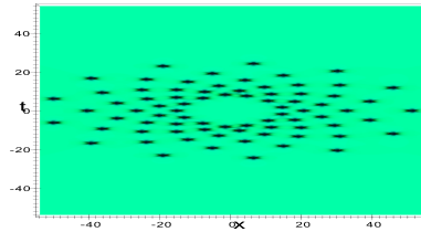
Figure 12: Solution of NLS, N=12 , \tilde{a}_6 = 10^{13} : 6 rings with 13 peaks without peak in the center; on the right, sight from top.
