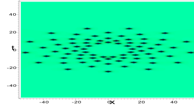
Figure 13: Solution of NLS, N=12 , \tilde{b}_6 = 10^{13} : 6 rings with 13 peaks without peak in the center; on the right, sight from top.
