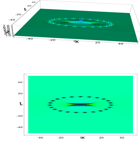
Figure 23: Solution of NLS, N=12 , \tilde{b}_{11} = 10^{20} : one ring with 23 peaks and in the center the Peregrine breather of order 10; on the right, sight from top.
