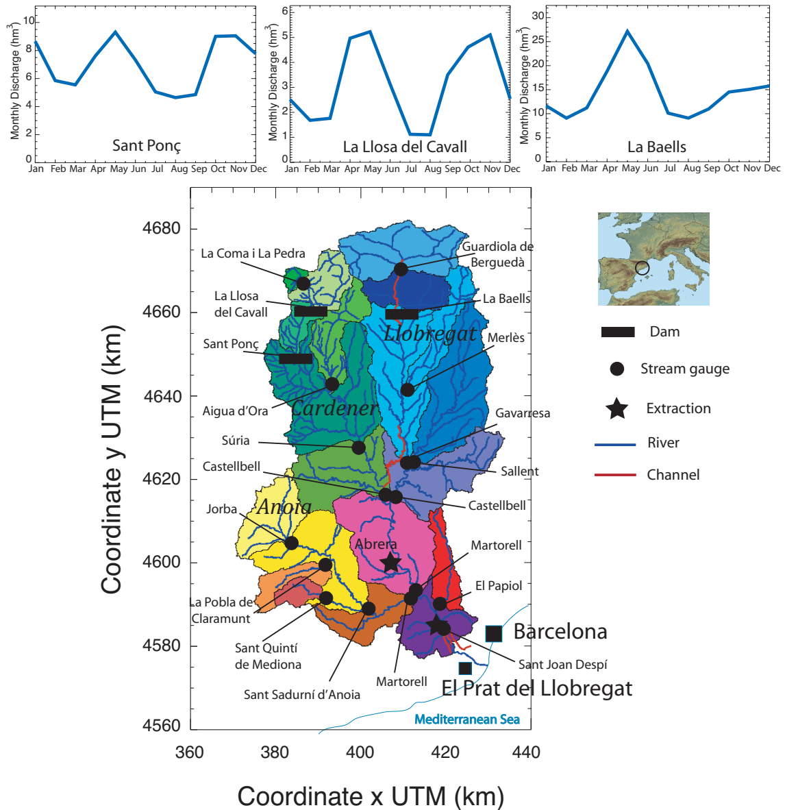
Fig. 1 The Llobregat basin disaggregated into sub-basins and the meteo-hydrographical network. Average monthly volumes (computed on the 1980-2010 time period) reaching the 3 dams are indicated.
