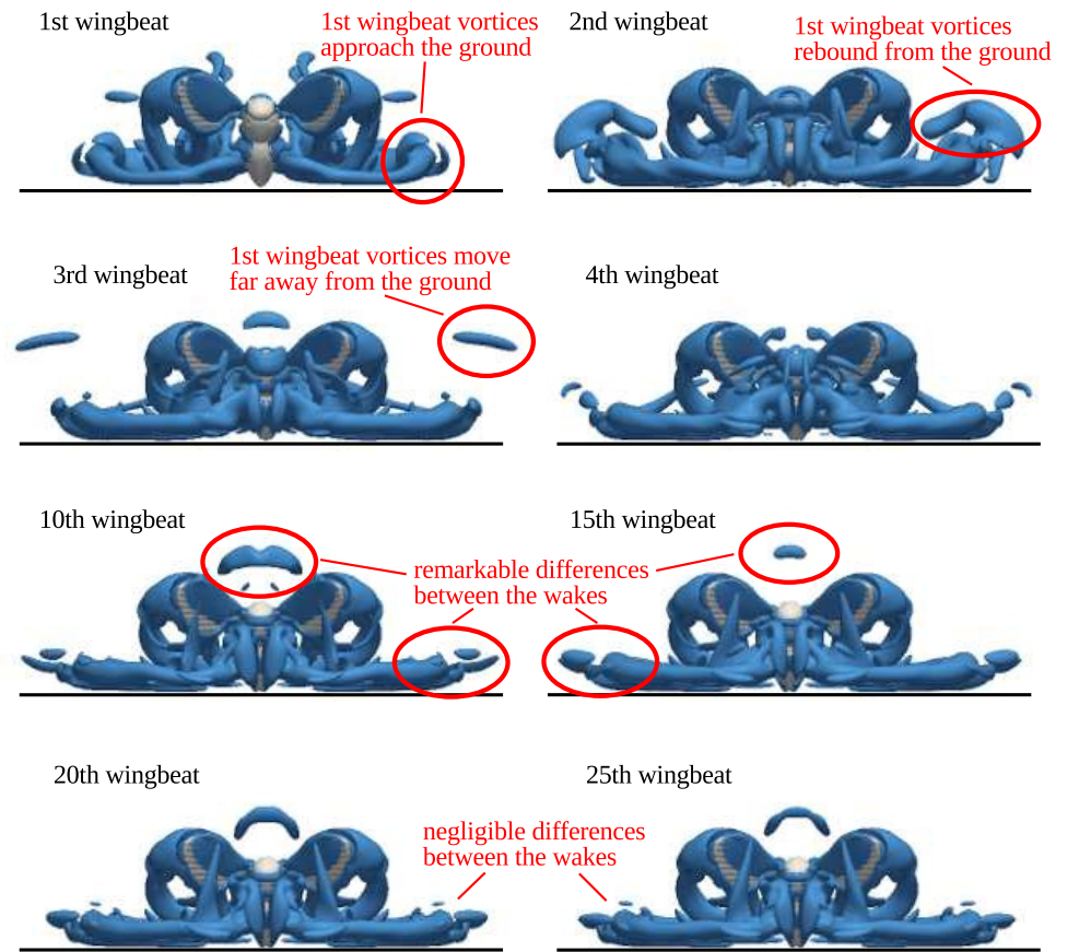
Fig 12. Time evolution of the wake during hovering. Iso-surfaces of the Q-criterion, Q/\rho^2 = 15 , are shown at the end of the downstroke. 'P1' kinematics with 100% wingbeat amplitude.
