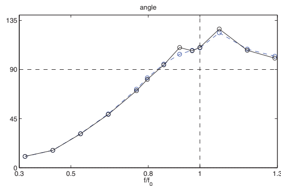
Figure 11: Maximum trailing edge deflection angle (averaged over strokes) as a function of f/f_0 for level 2 (blue dashed) and level 3 resolution (black). Dashed lines mark 90^\circ and the resonant frequency.
