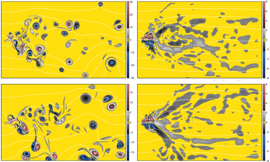
Figure 12: Two heaving foils in tandem, instantaneous (left) and time-averaged (right) vorticity fields. For visibility, only part of the computational domain is shown. The phase shift is \delta = 0.75\pi (top) and \delta = 1.25\pi (bottom).
