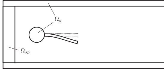
Figure 6: Setup for the benchmark proposed by Turek et al. [18]. A cylinder with an attached appendage is immersed in a channel configuration. The velocity sponge technique is used to impose a parabolic velocity profile in \Omega_{sp} . The appendage is either rigid (CFD test) or flexible (FSI test).
