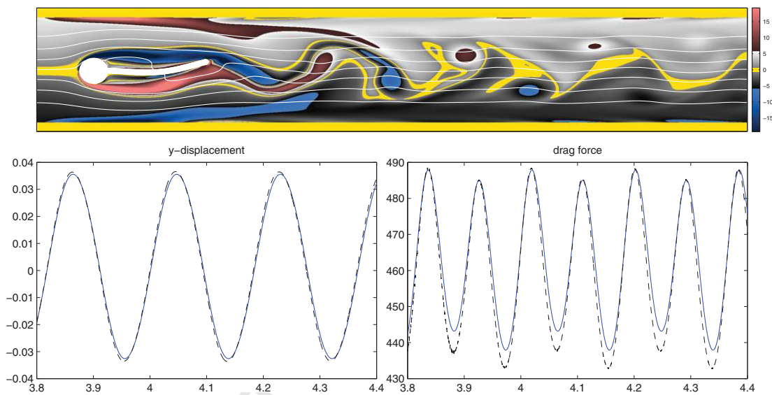
Figure 8: Results for the FSI3 test with a flexible appendage. Top: snapshot of the vorticity field with the deformed obstacle. Bottom: time series of the y-displacement of the trailing edge and of the drag force acting on the entire obstacle.
