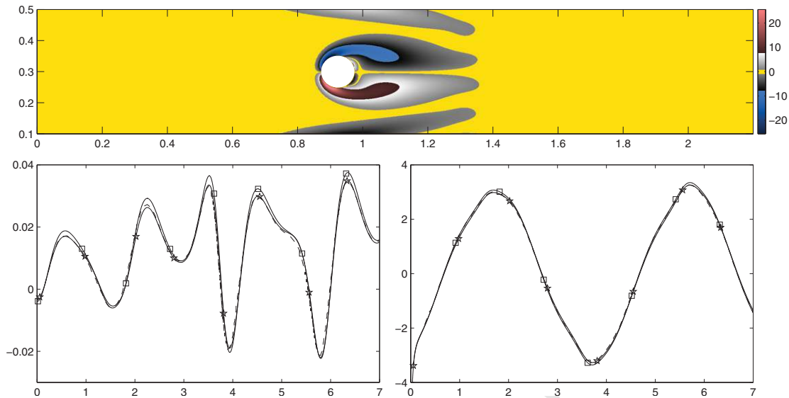
Figure 3: Hydrodynamic forces acting on an oscillating cylinder in a channel. Top: snapshot of the vorticity field. Bottom: lift (left) and drag force (right). Solid lines are present results ( 1024 \times 284 : \square , 2048 \times 568 : \star ) and results of Wan et al. [54] are represented by dashed lines.
