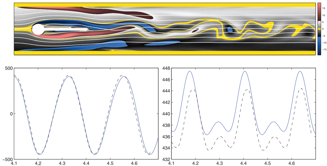
Figure 7: Results for the CFD3 test with rigid appendage. Vorticity field with stream lines and the obstacle (top). Bottom: time series of the lift (left) and drag force (right) on the obstacle. Present results are represented by blue solid lines and the reference solution [18] by the dashed black line.
