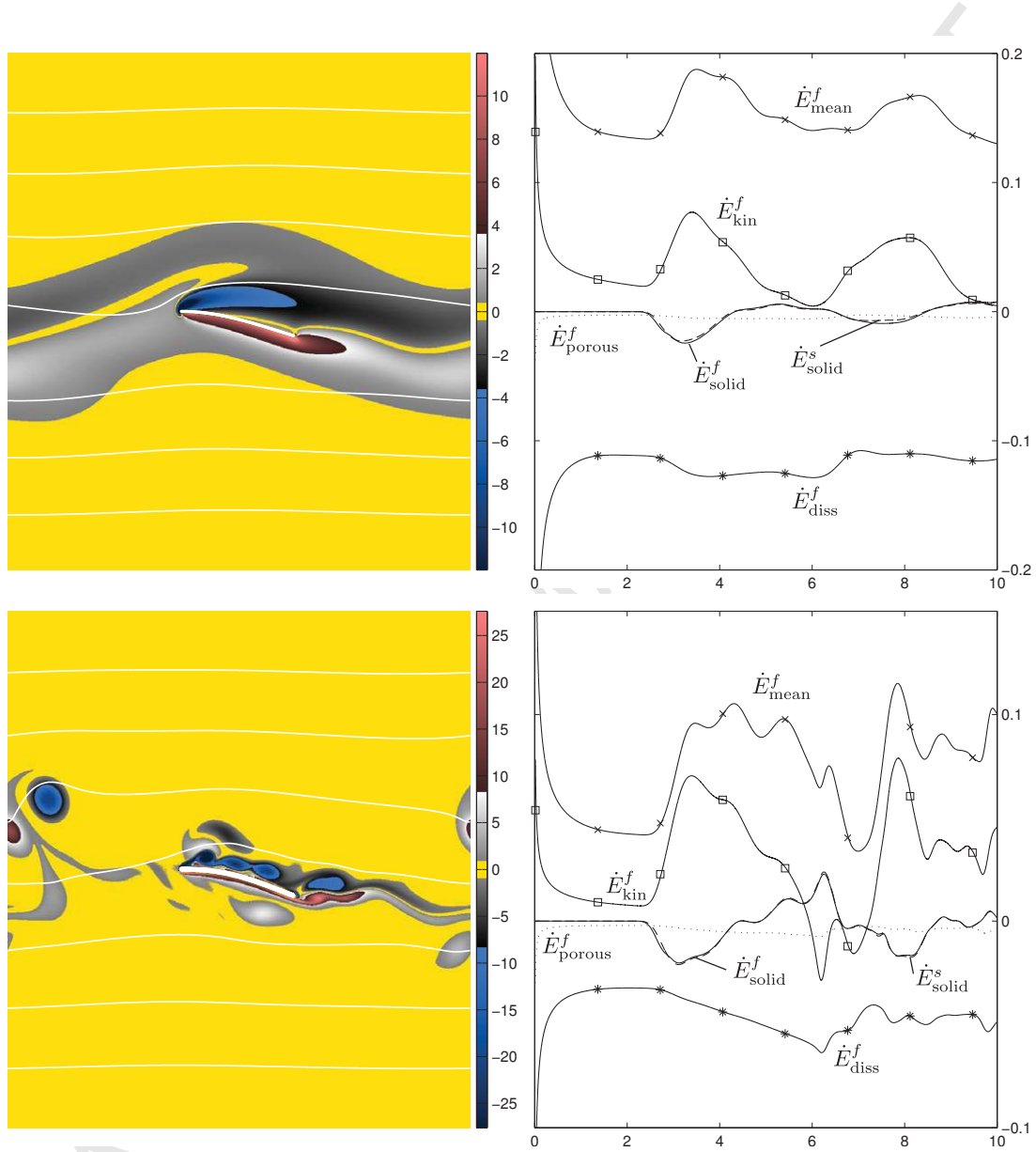
Figure 5: Energy test case for the Reynolds numbers 200 (top) and 2000 (bottom). Left column: Snapshot of the flow field, shown is vorticity with superimposed white streamlines. Right column: energy budget according to eqn. (34). The beam remains fixed until t = 2 . The startup singularity is due to the impulsively started flow. The curves for \dot{E}_{\text{solid}}^f and \dot{E}_{\text{solid}}^s show good agreement in both cases, indicating a good conservation of energy.
