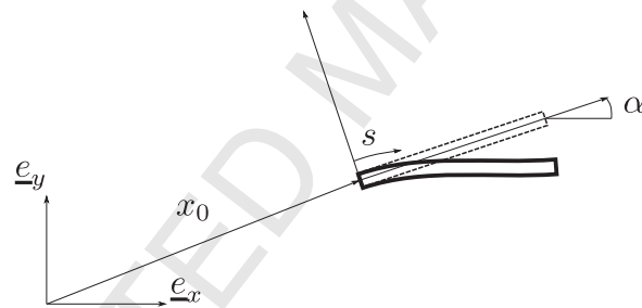
Figure 4: Illustration of the solid model used in the present work. The beam is clamped with respect to the relative coordinate system, which is translated by x_0 and rotated by \alpha .
