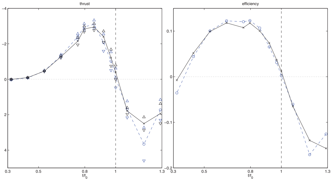
Figure 10: Thrust (left) and propulsive efficiency (right) as a function of the blackened heaving frequency f/f_0 . Curves for resolution level 2 (blue dashed) and 3 (black). Triangles indicate the 95% confidence interval, dashed line indicates the first resonant. The maximum thrust occurs at f/f_0 = 0.86 , which lies also in the region of maximum efficiency of about 12.5%.
