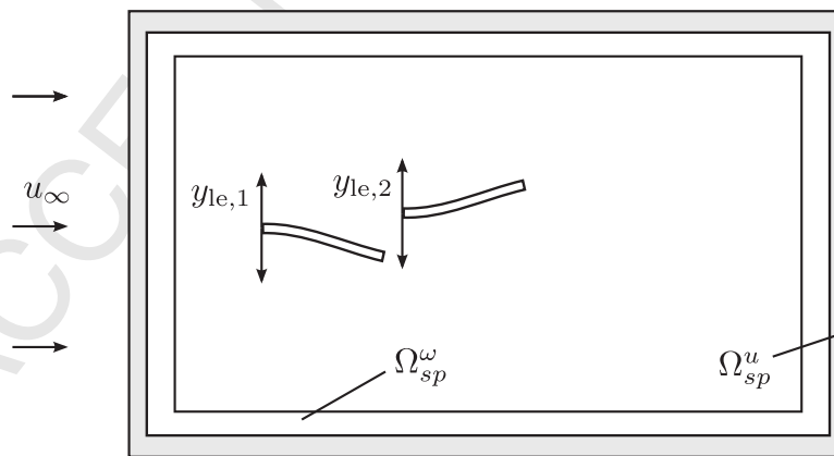
Figure 9: Setup for the wing section configuration. The flexible foils perform a sinusoidal heaving motion, and the second one is optional. The mean fluid flow u_{\infty} is imposed. A mixture of a \omega sponge and a u sponge is used. The \omega sponge damps incoming vortices slowly, in order to minimize the upstream influence. Remaining vorticity is then removed by the u sponge.
