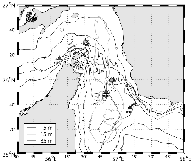
Figure 18. Surdrift buoy trajectories. Triangles indicate deployment position and colors give the drogued depth. Number of days of data is given in Table 3. See color version of this figure in the HTML.
