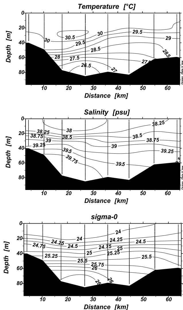
Figure 4. Cross-section R13c in the Arabian/Persian Gulf (location in Figure 3c) performed on 2 November 1999. Temperature, salinity, and potential density sections are shown. Vertical lines indicate cast positions.
