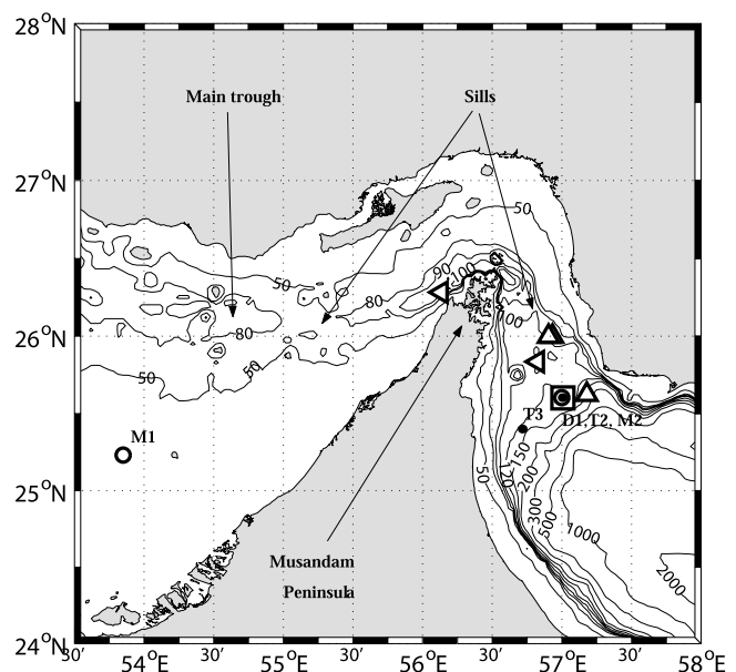
Figure 2. Bathymetry of the Strait of Hormuz and the Gulf of Oman from Etopo2 [Smith and Sandwell, 1997]. Mooring sites and drifting buoy deployments are indicated: dots for temperature recorders moorings T2 and T3, circles for tide recorders M1 and M2, squares for ADCP mooring D1, and triangles for initial deployment of drifters. Triangle orientations indicate drogues depth: 15 m (up) and 85 m (left).
