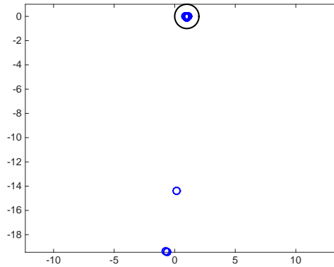
Figure 14: The spectrum of the ORAS-preconditioned matrix for k = 2 , \omega = \omega_2 , N_{\text{sub}} = 2 , \delta_{\text{ovr}} = 1h .
