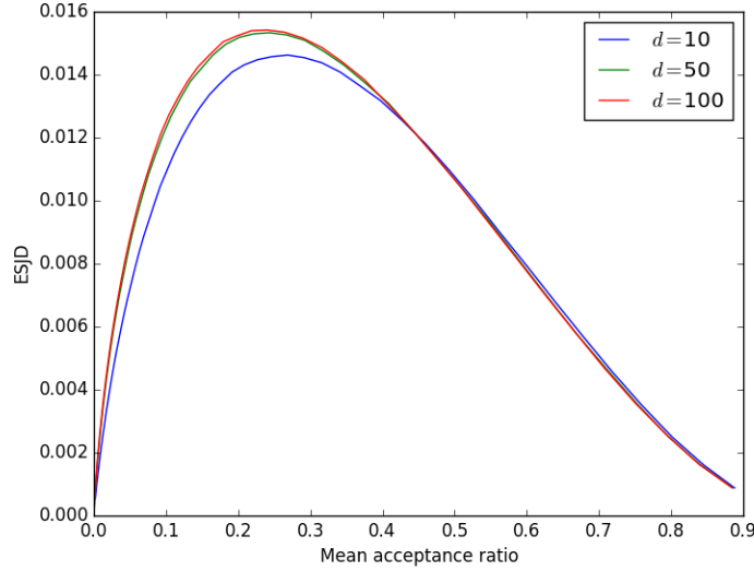
Figure 1: Expected square jumped distance for the beta distribution with parameters a_1 = 10 and a_2 = 10 as a function of the mean acceptance rate for d = 10, 50, 100 .
