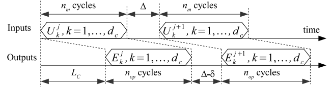
Fig. 4. Time diagram of a CNP. The d_c messages U of CN j are input in parallel in n_m clock cycles. After a latency of \Delta clock cycles, CN j + 1 performs.
