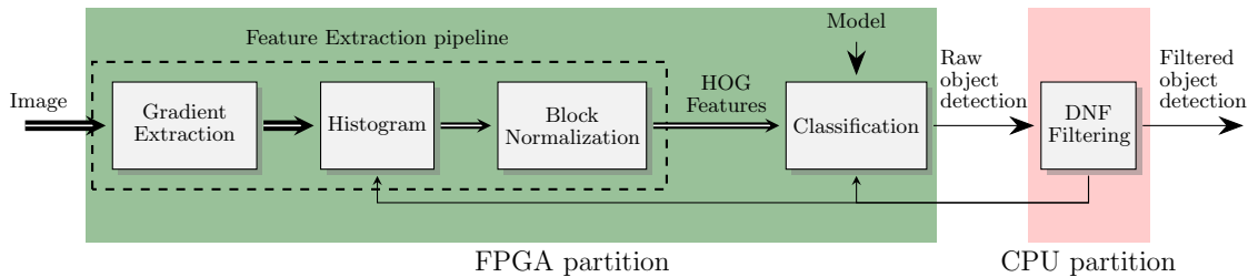
Fig. 3: Overview of the proposed hardware-software architecture.
