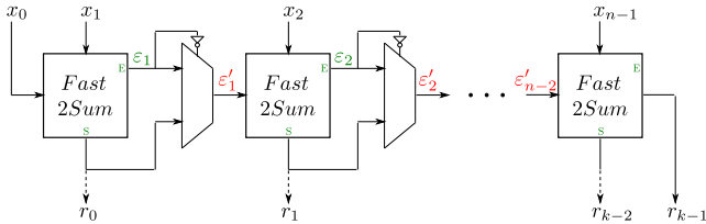
Fig. 2: Renormalize with n terms. Each Fast2Sum box performs an error-free transform; the sum is outputted downwards and the error-free transform to the right. If the sum is propagated to the right, otherwise the error is propagated and the sum is outputted.
