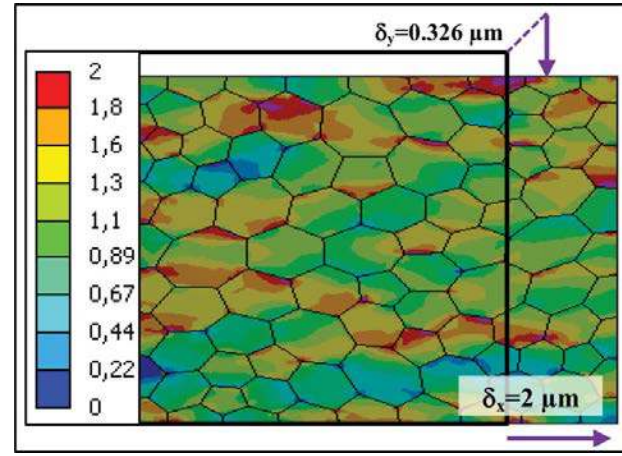
Figure 9. Mesoscopic normal stress, \sigma_x , distribution (MPa).
