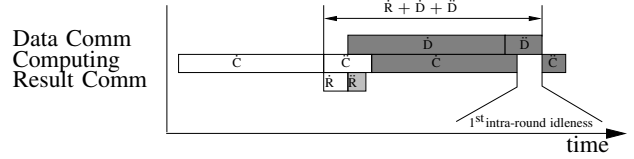
Fig. 10. Example of intra-round idleness with AS4DR
