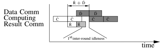
Fig. 9. Example of inter-round idleness with AS4DR
