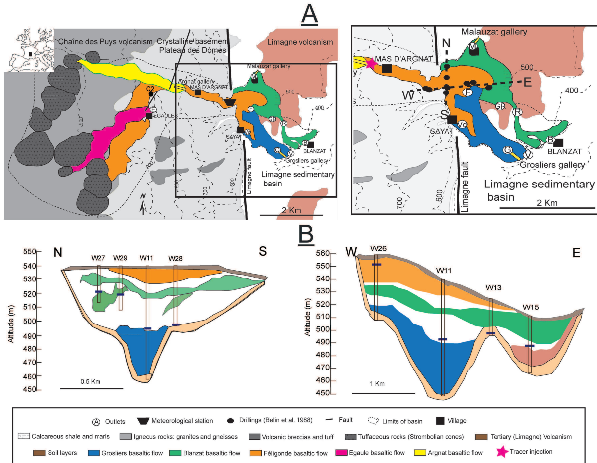
Figure 1: Location and geological settings of the Argnat basin; V: Vergnes, B: Blanzat, A: Argnat, E: Egaule, R: Reilhac catchment, Vd: Vernède, F: Féligonde, M: Malauzat, GR: Grande source de Reilhac, G: Grosliers.
