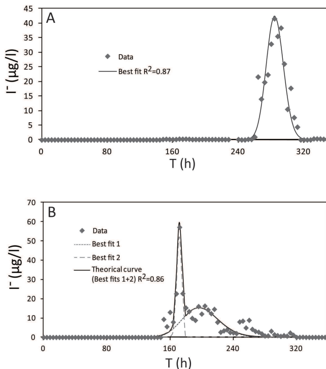
Figure 7: Single Fracture Dispersion Model (SFDM) applied for La Vernède (A) and Féligonde (B)'s tracer breakthrough curves.
