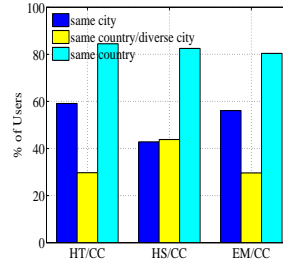
Fig. 1. User-centric Correlations
