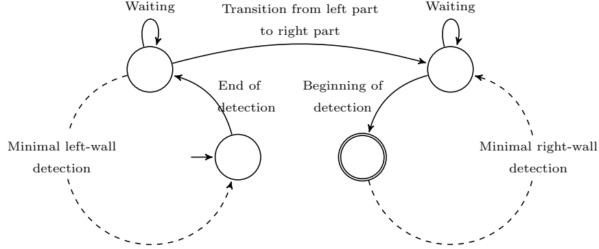
Figure 6: Conceptual view of the automaton \mathcal{A} .
