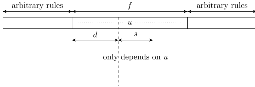
Figure 3: A strongly blocking word. Time goes downward.
