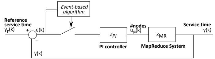
Fig. 13. Event-based PI feedback Control Architecture
