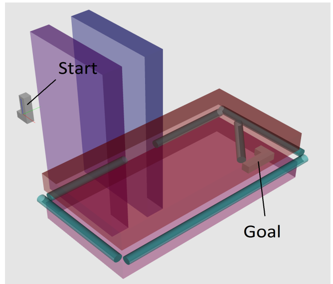
Fig. 7: Cluttered Space
