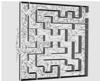
Fig. 5: RRT-connect
