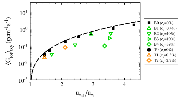
Figure 11. Total saltation flux \langle G_{tot} \rangle_{xy} as a function of the saltation friction velocity over an equivalent bare sand u_{s, sb} normalized by the threshold friction velocity u_{*t} , deduced from all simulated cases. The dashed black line fits dots of the bare sand case B0 ( \langle G_{tot} \rangle_{xy} = c \sqrt{\langle d_p \rangle} / D \rho u_{s, sb}^3 (1 - u_{*t} / u_{s, sb}) / g with D = 250 \mu\text{m} and c = 1.8 for \langle G_{tot} \rangle_{xy} in kilogram per meter per second).
