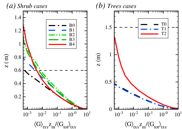
Figure 8. Vertical profiles of the mean saltation flux \langle G \rangle_{xy} ( \text{g cm}^{-2} \text{ s}^{-1} ) normalized by the total saltation flux \langle G_{tot} \rangle_{xy} ( \text{g cm}^{-1} \text{ s}^{-1} ) and by the saltation layer height z_m , for (a) shrub and (b) tree cases. Cases B0 and B2 correspond to simulations with u_{*sb} = 0.54 and 0.90 \text{ m s}^{-1} , respectively. The dashed lines represent the shrub top (Figure 8a) and the lower tree crown level (Figure 8b).
