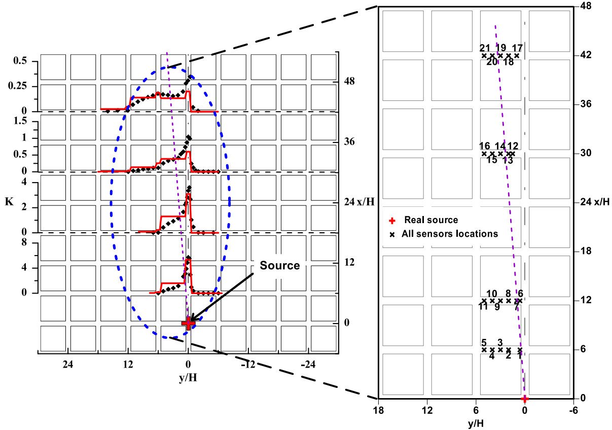
Fig. 1a. Comparison between experimental results (diamonds) and numerical results (lines) at different distances from the source, (placed at +). The dashed line indicates the wind direction of the external wind ( 12.5^\circ ). Fig. 1b. Position of the receptors used in the inverse modelling.
