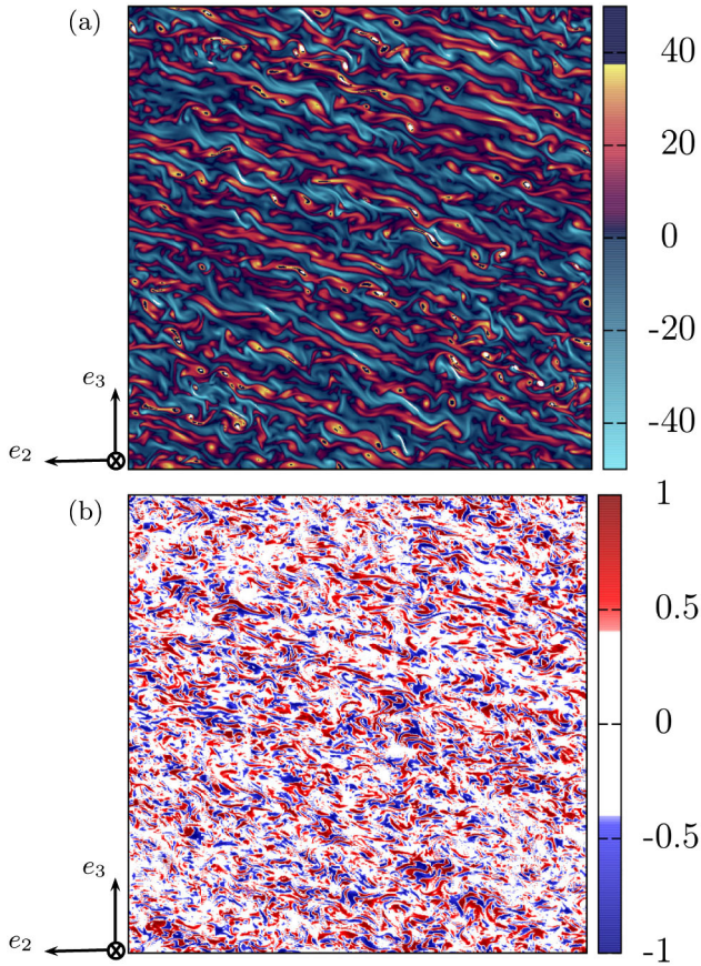
FIG. 5 (color online). (a) Zonal vorticity in the vertical or meridional plane at time tS = 20 , run A. (b) The corresponding distribution of \cos \tilde{\theta} defined in Eq. (10). The slope of the vortical structures is approximately 24.5^\circ , which is close to the baroclinic angle \arctan(N_h^2/N_v^2) = 26.6^\circ .
