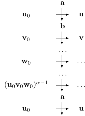
■ Figure 2 Extension of Property ( Ubiquity ) from \mathbf{u}_0 to \mathbf{u} .
