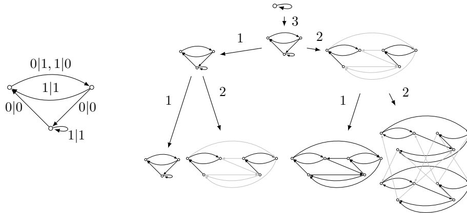
■ Figure 1 The Bellaterra automaton \mathcal{B} and four levels of the orbit tree t(\mathcal{B}) .
