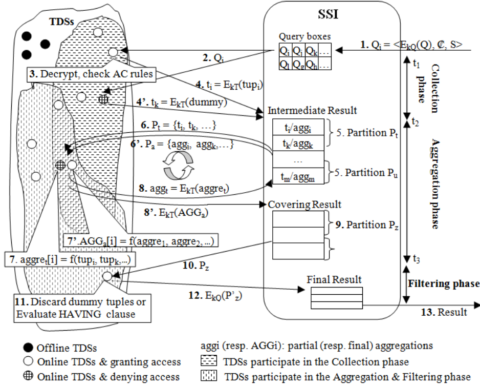
Fig. 5. Group By querying protocol
