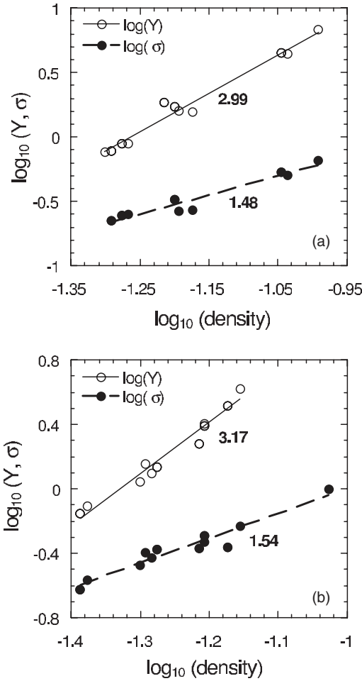
FIG. 7. Examples of the log-log plots of the Young's modulus Y and compressive strength \sigma as functions of the density. (a) Samples that were heat-treated at 200°C and measured in the xy plane. (b) Samples that were heat-treated at 800°C and measured along the z direction. The straight lines represent linear fits of the data with their slopes.
