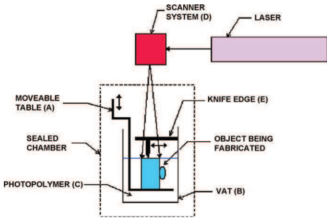
Fig. 3. Stereolithography.
