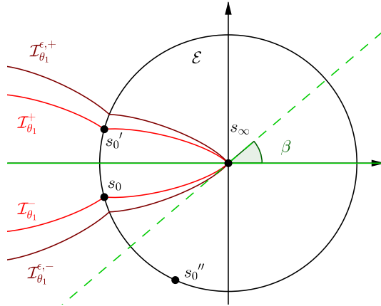
FIGURE 12. \mathcal{I}_{\theta_1}^{\epsilon,-} and \mathcal{I}_{\theta_1}^{\epsilon,+}
