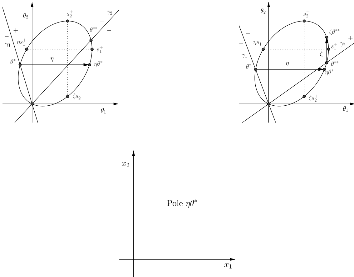
FIGURE 21. Theorem 26 case (iiia) and (ivb)
