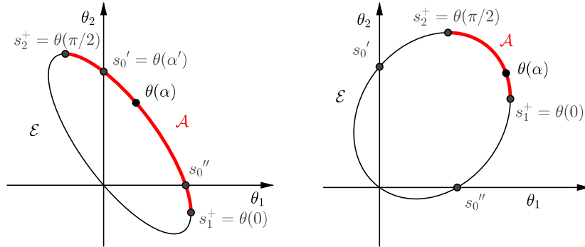
FIGURE 18. The arc \mathcal{A} = [s_1^+, s_2^+] if \theta_1(s_2^+) < 0 , \theta_2(s_1^+) < 0 on the left picture, if \theta_1(s_2^+) > 0 , \theta_2(s_1^+) > 0 on the right picture
