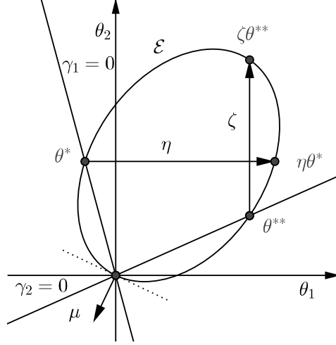
FIGURE 2. Ellipse \mathcal{E} , straight lines \gamma_1(\theta) = 0 , \gamma_2(\theta) = 0 , points \theta^* , \theta^{**} , \eta\theta^* , \zeta\theta^{**}
