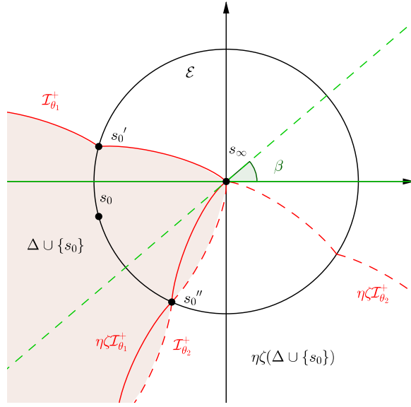
FIGURE 11. \Delta and \eta\zeta\Delta
