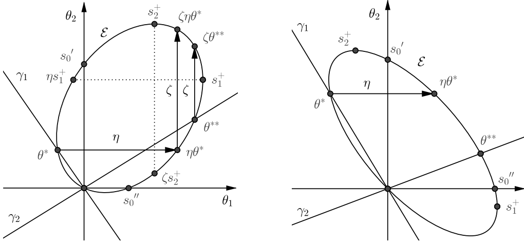
FIGURE 13. On the left figure : \eta\theta^* is the closest pole of \varphi_1 to s''_0 on ]s''_0, s_2^+[ , \zeta\eta\theta^* is the closest pole of \varphi_2 to s'_0 on ]s_1^+, s_0[ . On the right figure: \eta\theta^* is the closest pole of \varphi_1 to s''_0 on ]s''_0, s_2^+[ , there are no poles of \varphi_2 on ]s_1^+, s'_0[
