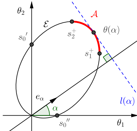
FIGURE 3. Arc \mathcal{A} and point \theta(\alpha) on \mathcal{E}
