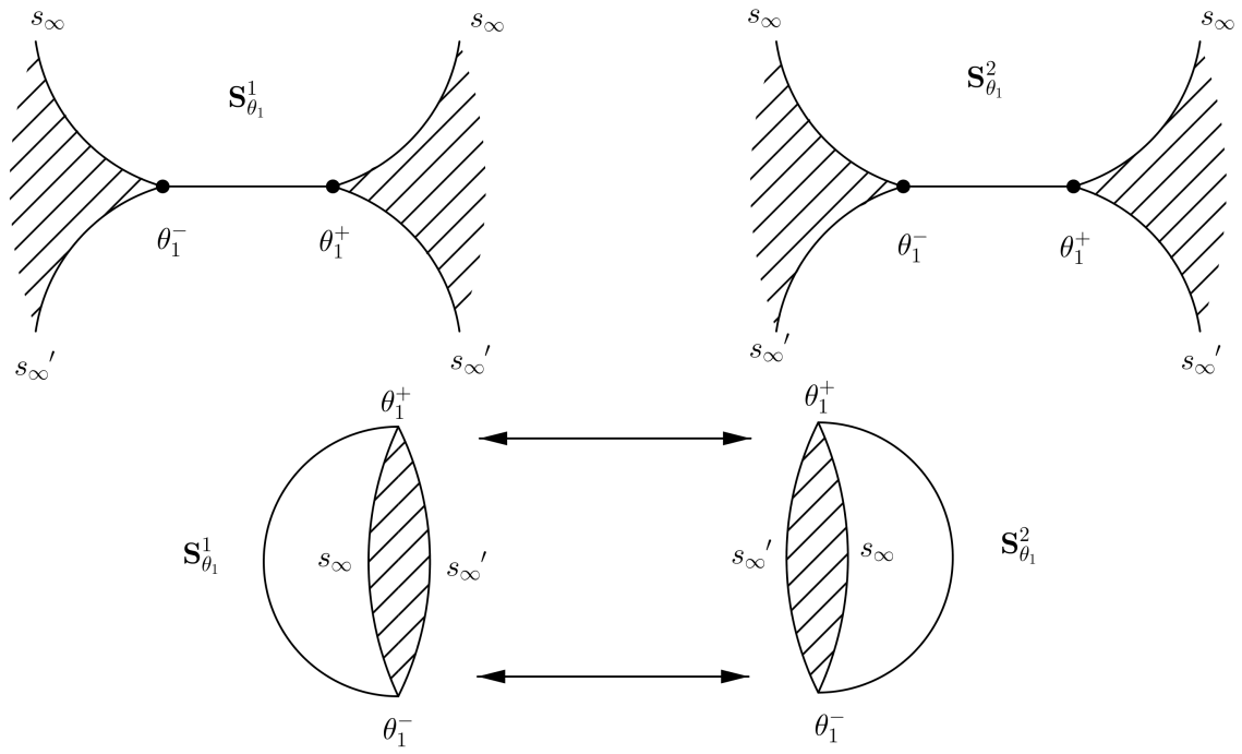
FIGURE 6. Construction of the Riemann surface \mathbf{S}
