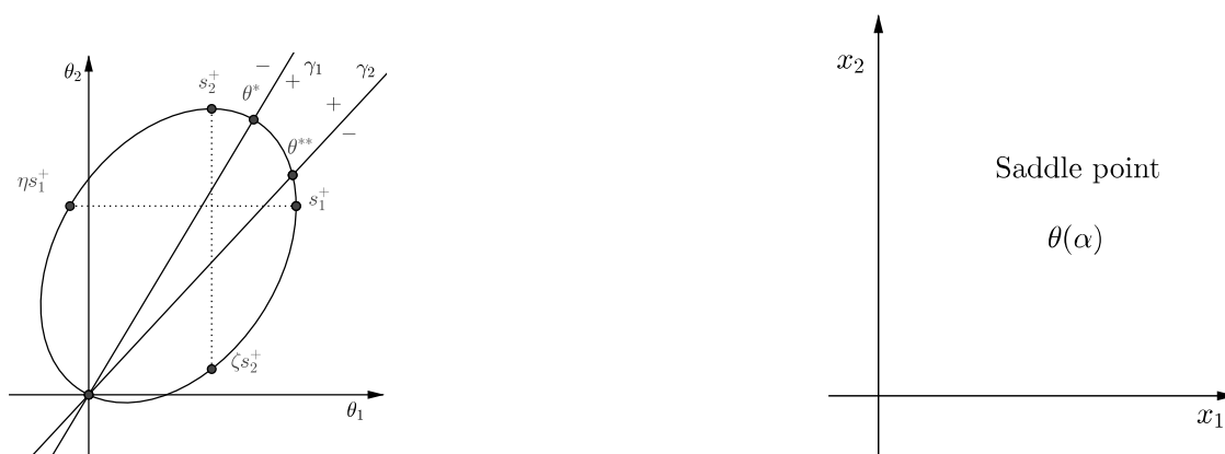
FIGURE 19. Theorem 26 case (i)
