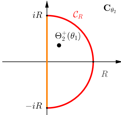
FIGURE 14. Contour \mathcal{C}_R on \mathbf{C}_{\theta_2} .
