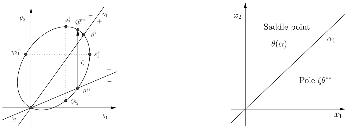
FIGURE 22. Theorem 26 case (iib)
