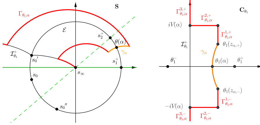
FIGURE 16. Contour \Gamma_{\theta_1, \alpha} on parametrized \mathbf{S} and projected on \mathbf{C}_{\theta_1} .
