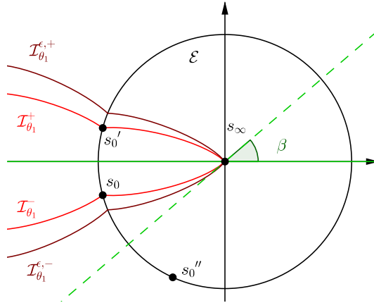
FIGURE 12. \mathcal{I}_{\theta_1}^{\epsilon,-} and \mathcal{I}_{\theta_1}^{\epsilon,+}
