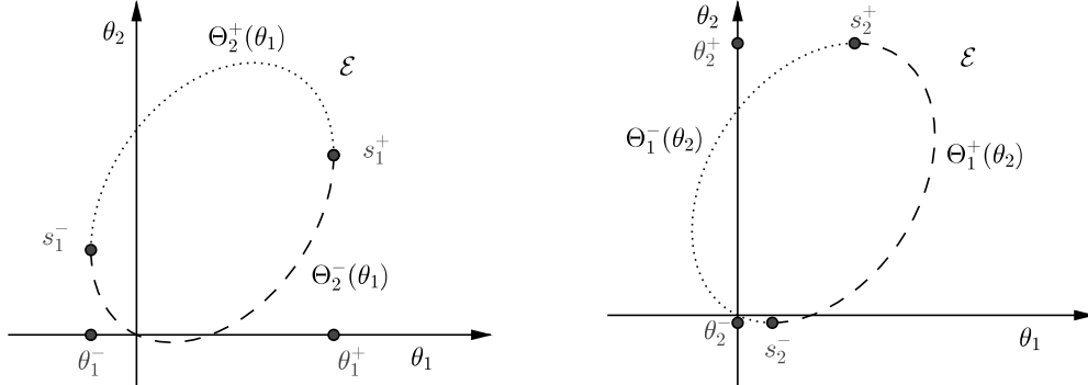
FIGURE 5. Functions \Theta_2^\pm(\theta_1) and \Theta_1^\pm(\theta_2) on [\theta_1^-, \theta_1^+] and [\theta_2^-, \theta_2^+]
