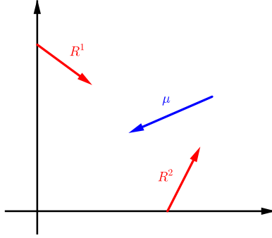
FIGURE 1. Drift \mu and reflection vectors R^1 and R^2
