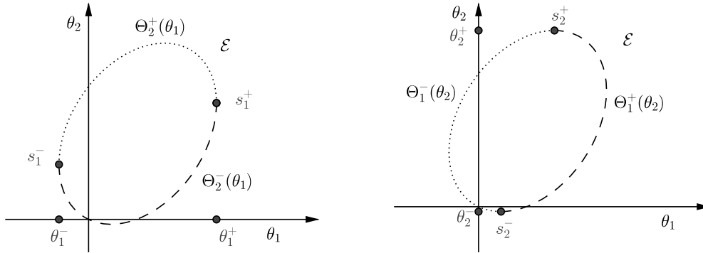
FIGURE 5. Functions \Theta_2^\pm(\theta_1) and \Theta_1^\pm(\theta_2) on [\theta_1^-, \theta_1^+] and [\theta_2^-, \theta_2^+]
