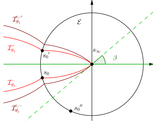
FIGURE 12. \mathcal{I}_{\theta_1}^{\epsilon,-} and \mathcal{I}_{\theta_1}^{\epsilon,+}
