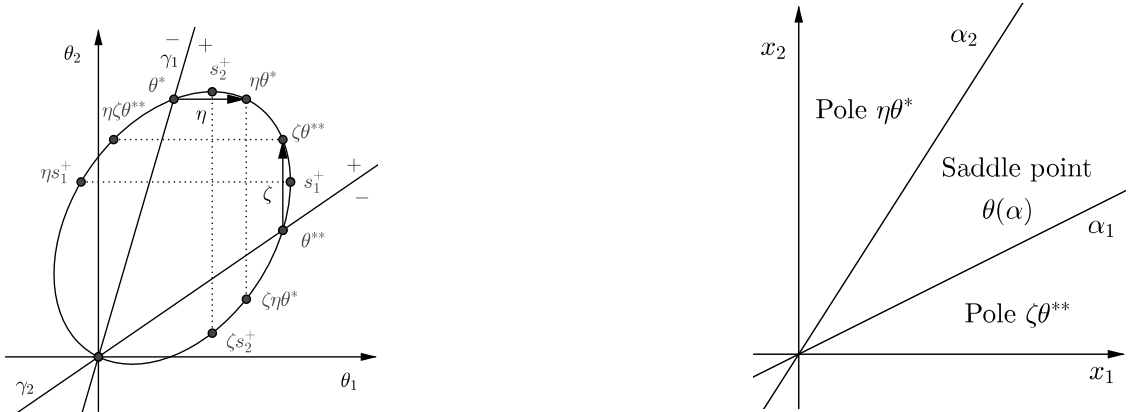
FIGURE 25. Theorem 26 case (ivd)
