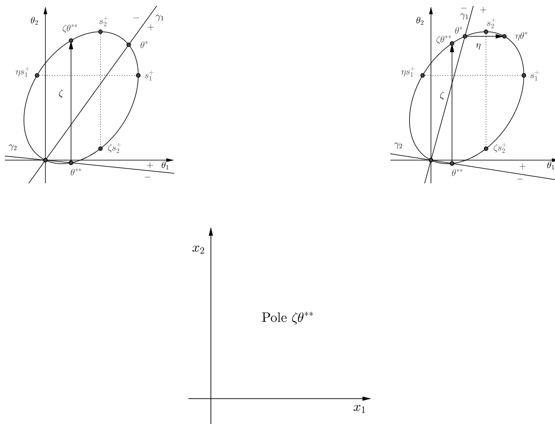
FIGURE 20. Theorem 26 case (ia) and (iva)
