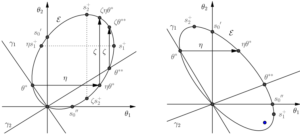
FIGURE 13. On the left figure : \eta\theta^* is the closest pole of \varphi_1 to s_0'' on ]s_0'', s_2^+[ , \zeta\eta\theta^* is the closest pole of \varphi_2 to s_0' on ]s_1^+, s_0'[ . On the right figure: \eta\theta^* is the closest pole of \varphi_1 to s_0'' on ]s_0'', s_2^+[ , there are no poles of \varphi_2 on ]s_1^+, s_0'[
