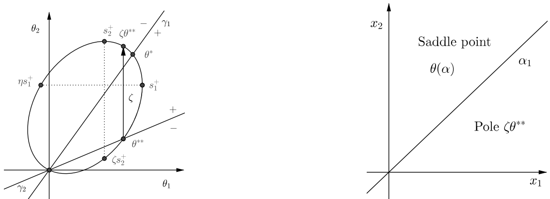
FIGURE 21. Theorem 26 case (iiia) and (ivb)
