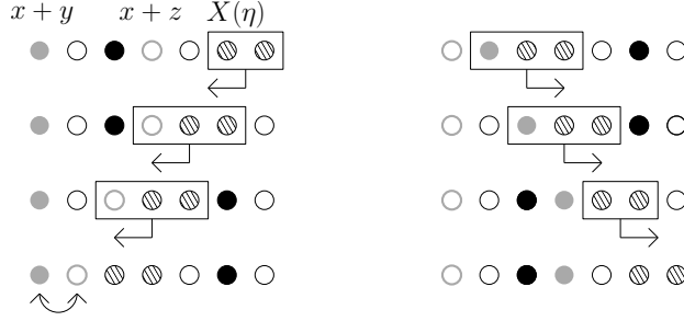
FIGURE 2. How to construct the wanted path for the case \eta(X(\eta))\eta(X(\eta)+1) = 1 (in the other case, start by making the particle at X(\eta)+2 jump left). The hole and particle that we want to exchange are in gray, the mobile cluster in stripes and the rest of the configuration in black. By exchanging X(\eta)-1, X(\eta) , then X(\eta), X(\eta)+1 we move the mobile cluster one step to the left. Similarly, we move the group {gray hole, striped particles} to the left until it touches the gray particle. Exchange the gray hole and particle and retrace the steps back.
