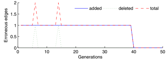
Figure 12: Evolution of the number of erroneous edges of the structure along generations
