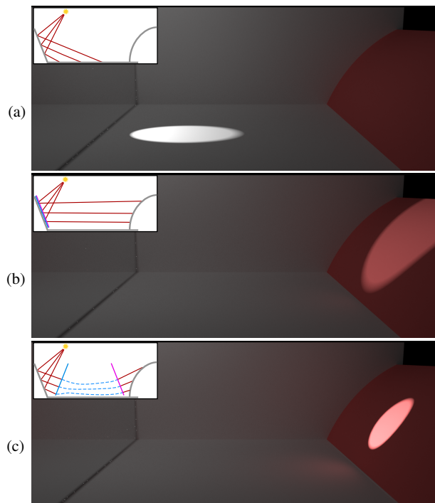
Fig. 8 Application of Figure 4. (a) Original rendering. (b) Light retargeting with portals. (c) Light field teleportation with portals.
