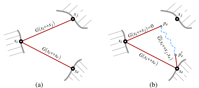
Fig. 3 (a) Non-edited scene, where the light propagation along segments \langle x_i, x_j \rangle and \langle x_i, x_e \rangle is computed using G . (b) Edited scene: propagation along \langle x_i, x_j \rangle is cancelled at p_e , and transformed to p'_e in order to finally fall on x_e . This whole process is defined by the edited propagation term \bar{G} . Red lines represent propagation segments, potentially shared between multiple lightrpaths.
