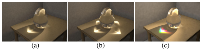
Fig. 9 A portal captures the caustic and replicates it with multiple output surfaces, disposed around the glass egg. (a) Original scene. (b) Duplication. (c) Duplication and shifting spectrum hue.
