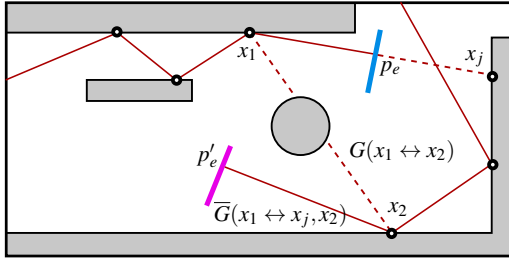
Fig. 5 When evaluating the propagation between two points, we need to take portals into account. Here, G(x_1 \leftrightarrow x_2) is nil but going through the portals, a shadow ray lands on x_2 and transmits light from x_1 to x_2 .
