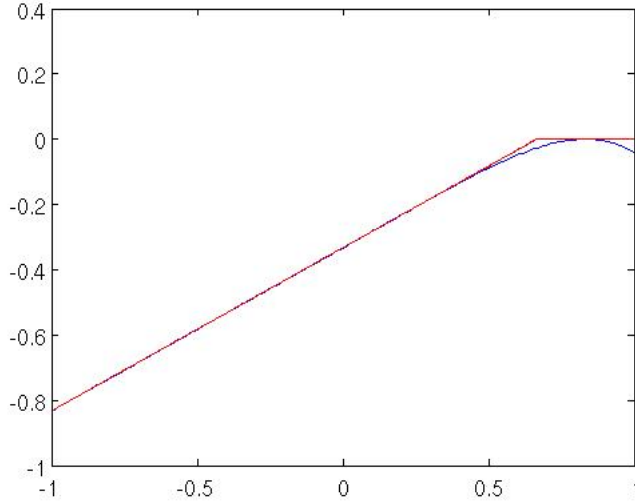
FIG. 1. J(x) and its degree-6 underestimation in Example 4.8.
