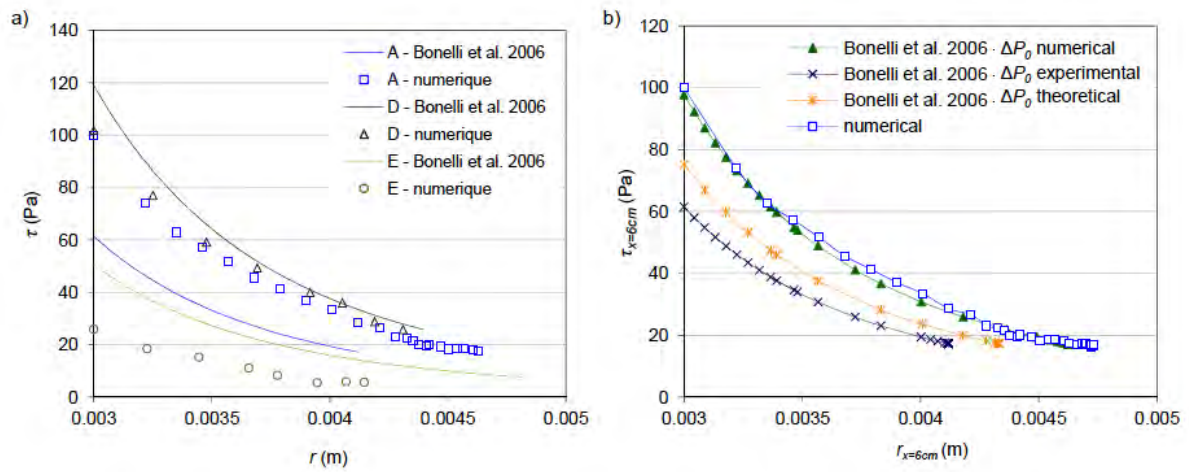
Fig. 8 Evolution of a) the shear stress for the three tests and b) the shear stress in case of soil A for the different \Delta P_0 , as a function of the radius reached, values taken in the middle of the erodible channel
