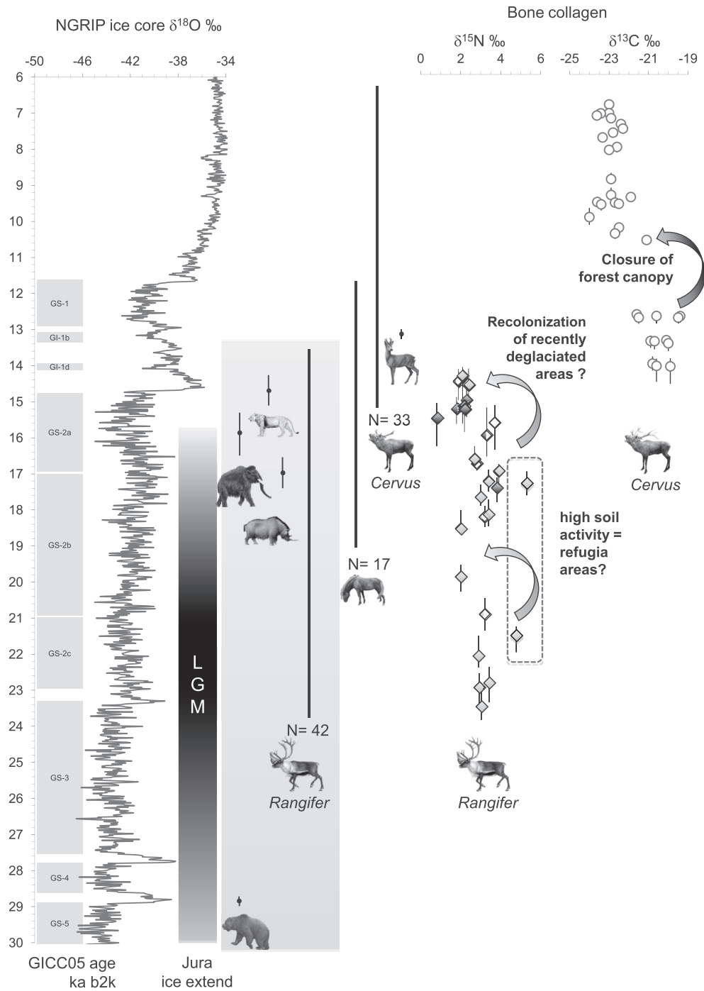
Fig. 3. AMS radiocarbon and isotopic records of selected fauna species from the Jura area. The latest date (2 sigmas) is given for the extinct species ( Panthera leo , Stuart and Lister, 2011; Bocherens et al., 2011; Coleodonta antiquitatis , Cupillard and Welté, 2009; Mammuthus primigenius , Bridault and Chaix, 2009). The earliest date is given for Capreolus capreolus , unpubl. For the three other herbivore hunted species, Rangifer tarandus , Equus ferus and Cervus elaphus , the time range is given as well as the number of dates. The bone collagen \delta^{15}\text{N} values of reindeer over time reflect the intensity of soil processes which depends mainly on the temperature and permafrost influence (e.g. Drucker et al., 2012). Increasing soil activity as a result of decreasing permafrost intensity lead to increasing \delta^{15}\text{N} values in soils, plants and animals of the ecosystem. The diamonds in dark grey correspond to reindeer remains found in archaeological sites that were not accessible during the main part of the Last Glacial Maximum. The bone collagen \delta^{13}\text{C} values of red deer are an indicator of the density of the forest cover. Under a dense canopy, the depleted \delta^{13}\text{C} values of plants are passed on to the large herbivores feeding regularly on them (e.g. Drucker et al., 2008, 2011a). (For interpretation of the references to colour in this figure legend, the reader is referred to the web version of this article.)
