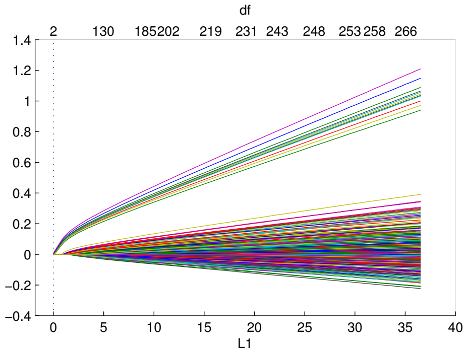
Trace Plot of coefficients fit by Lasso
