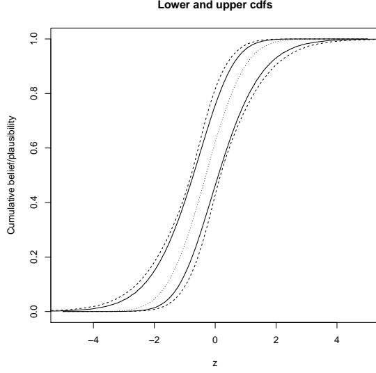
Figure 5: Lower and upper cdf for the normal data (Example 6): exact bounds (solid lines), approximations using the marginal contour functions (interrupted lines) and plug-in cdf \Phi((z - \bar{y})/s^2) (central dotted line).
