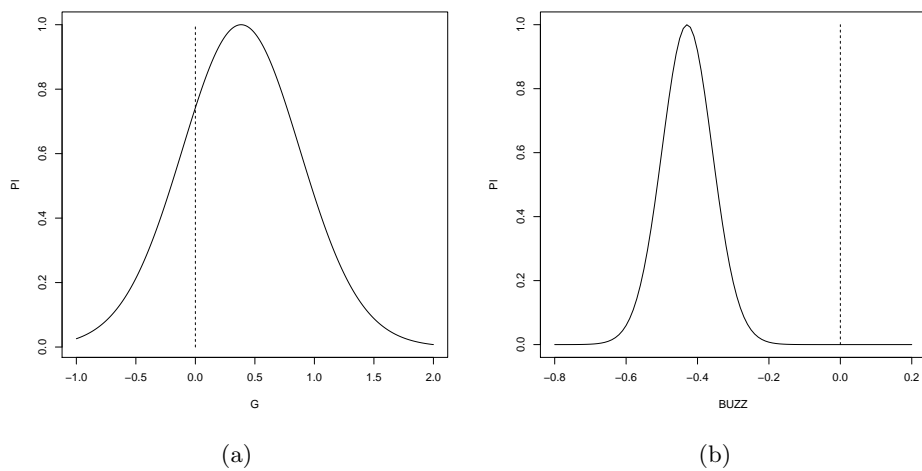
Figure 6: Marginal contour functions for the coefficients of variables G (a) and BUZZ (b).
