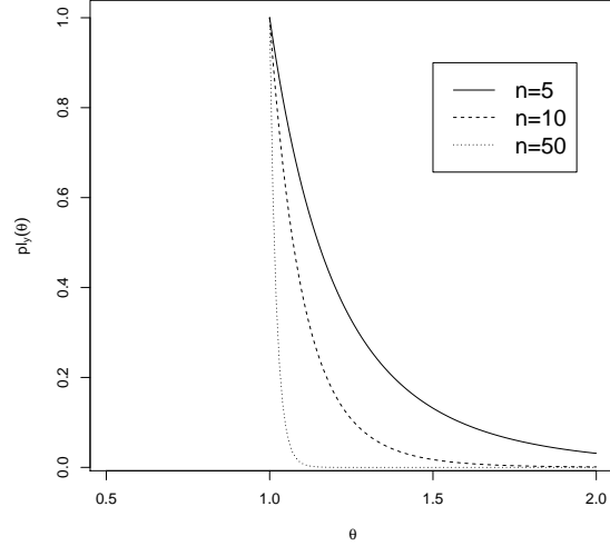
Figure 1: Contour function on \theta for an iid sample from \mathcal{U}([0, \theta]) , with y_{(n)} = 1 and n \in \{5, 10, 50\} .
