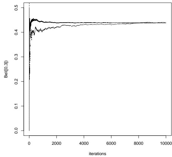
Figure 4: Example of convergence of \widehat{Bel}_y^Z([0, 3]) to Bel_y^Z([0, 3]) for Halton draws (upper solid line) and random draws (lower interrupted line) from a uniform distribution.
