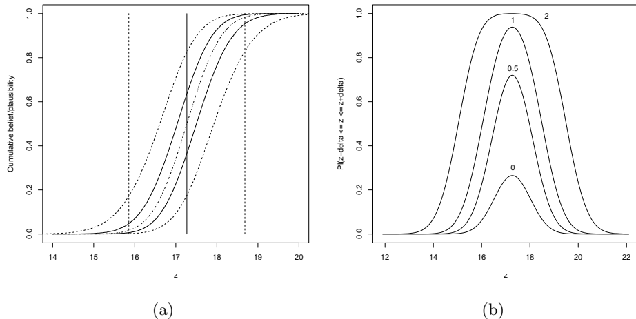
Figure 7: (a): Lower and upper cdf for the prediction problem: exact values (solid lines) and outer approximations (interrupted lines); the central curve is the cdf of the plug-in distribution of Z ; the vertical dotted lines correspond to the frequentist 95% prediction interval. (b): pl-plot: plausibility Pl_{\mathbf{y}}^{\mathbb{Z}}([z - \delta, z + \delta]) as a function of z , for \delta \in \{0, 0.5, 1, 2\} .
