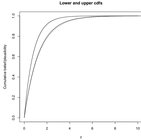
Figure 3: Lower and upper cdf for the exponential data (Example 5): exact bounds (plain curves) and normal approximations (dotted curves)
