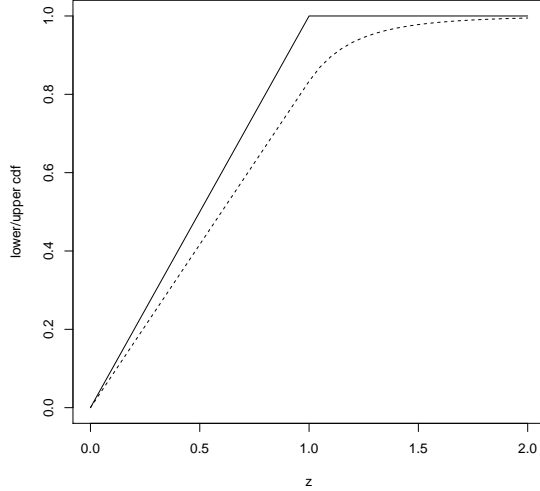
Figure 2: Lower and upper predictive cdf for y_{(n)} = 1 and n = 5 (Example 4).
