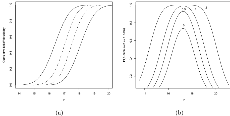
Figure 8: (a): Lower and upper cdf for the prediction problem with uncertain inputs (solid lines) and with certain inputs (interruption lines); (b): pl-plot of the predictive belief function with uncertain inputs.
