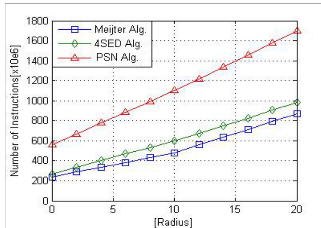
Fig.6: Comparison between different EDT algorithms
