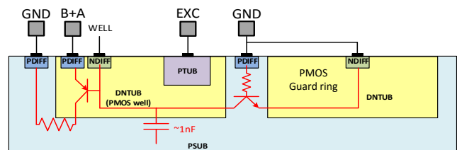
Figure 5 Example of substrate parasitic hand extraction
