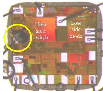
Figure 4 AUTOCHIP1 damage after battery connection
