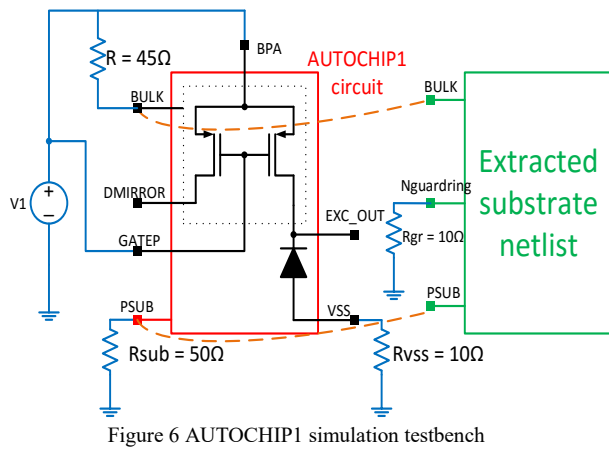
Figure 6 AUTOCHIP1 simulation testbench
