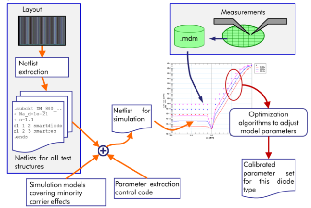
Figure 2 technology parameters extraction flow
