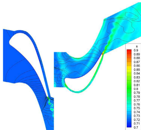
(b) Third order RBCi scheme
