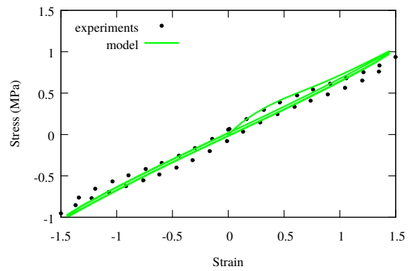
(b) Tension at \theta = 20^\circ C
