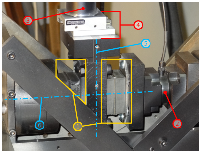
Figure 17: laminated bearing setup for dynamical shear test with static compression.
