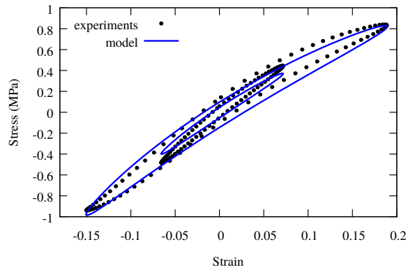
(d) Tension/Compression at f = 3Hz, \theta = -40^\circ C
