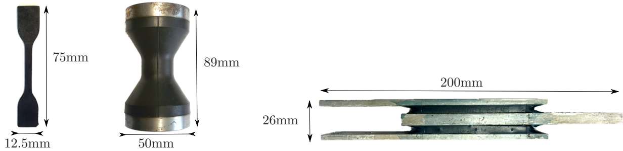
Figure 2: Specimens, left from right: H2, diablo and double-shear.
