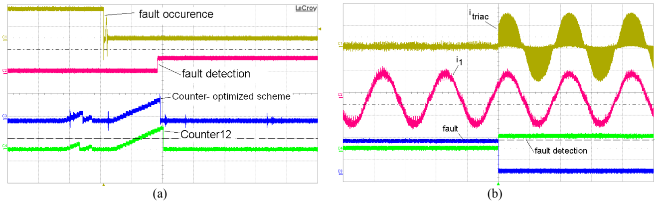
Fig. 16. (a) Comparison of the detection signals without and with the optimization, (x-axis: 20 \mu s/div ) (b) current of the phase 1 and the current of the corresponding TRIAC (y-axis: 5A/div ; x-axis: 10 ms/div ).
