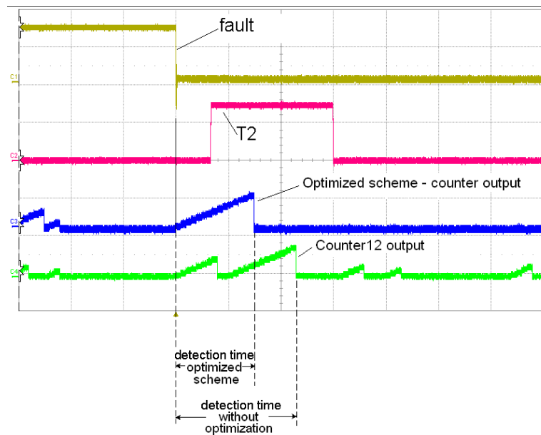
Fig. 17. Comparison of the fault detection times without and with the optimization for a fault in S1 and a transition in T2 during the fault detection.(y-axis from top to bottom: 10V/div , 10V/div , 33/div , 33/div ; x-axis: 20 \mu s/div )
